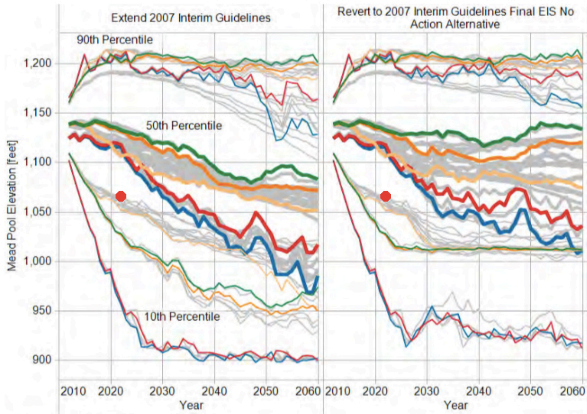
FIGURE G-6 10th, 50th, 90th Percentiles for Lake Mead End-of-December Pool Elevation
