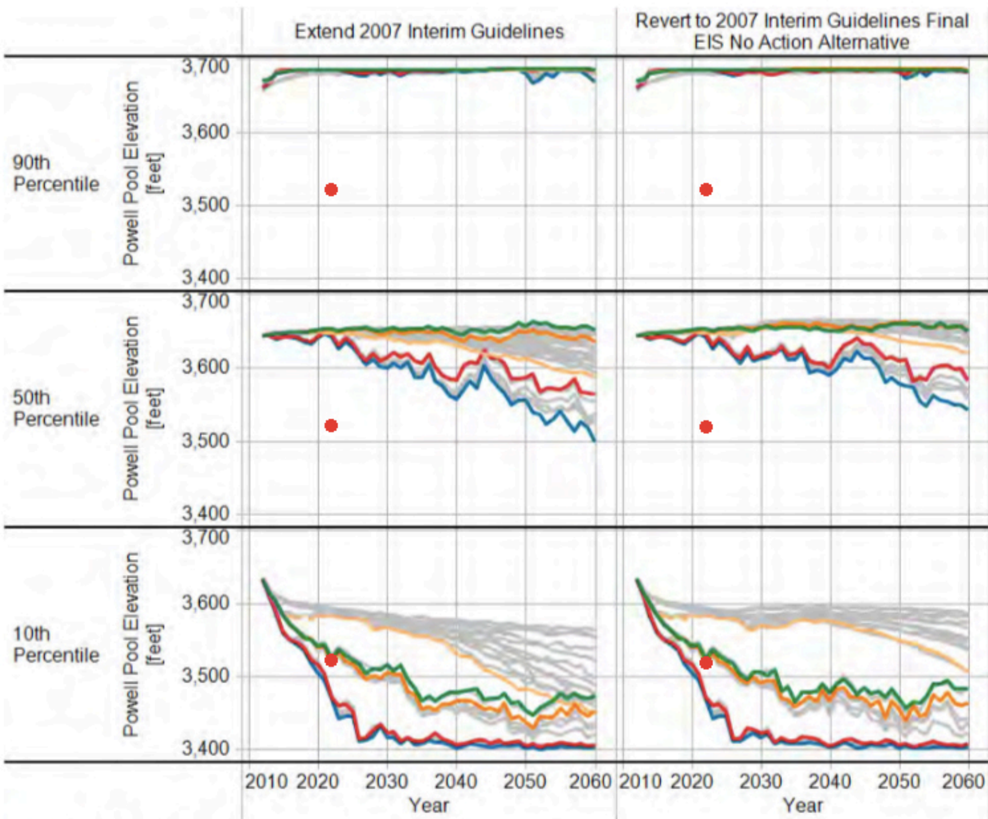
FIGURE G-4 10th, 50th, 90th Percentiles for Lake Powell End-of-December Pool Elevation
