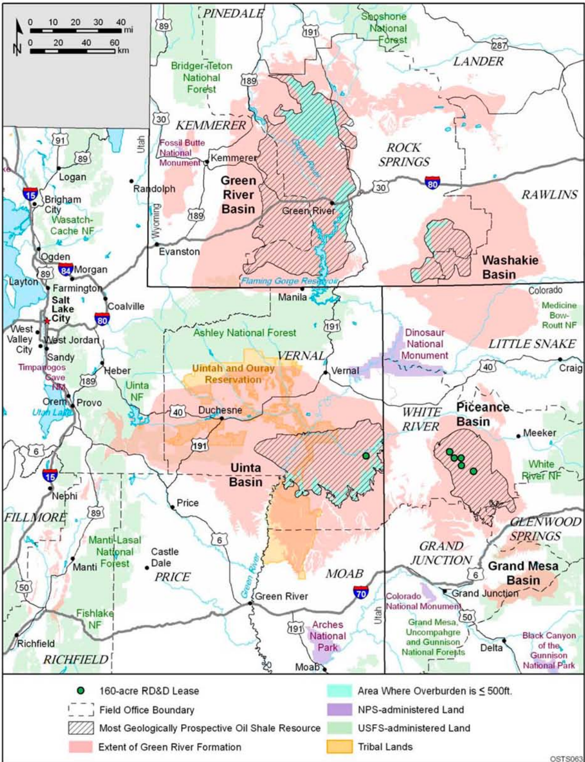
Green River Formation Basins in Colorado, Utah, and Wyoming; the Most Geologically Prospective Oil Shale Resources; the Areas Where the Overburden above the Oil Shale Resources Is \leq 500 ft; and Locations of the Six RD&D Projects
