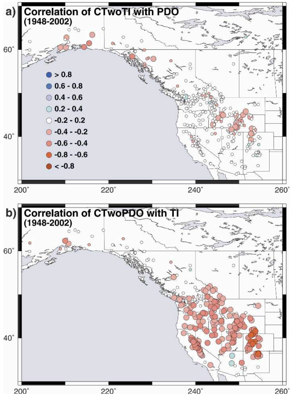
FIG. 11. Correlation of (a) CT minus the portion of its variance attributable to the TI (CTTwoTI), with PDO and (b) CT minus the portion of its variance attributable to the PDO index (CTTwoPDO), with TI. The larger symbols indicate statistically significant correlations at the 95% confidence level.
