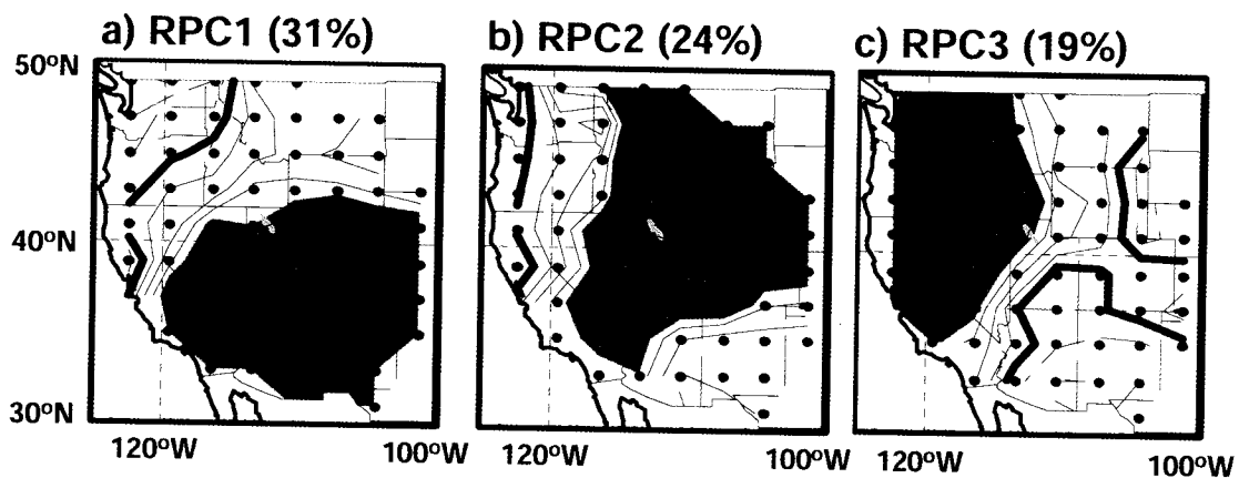
Figure 4. Loadings of the first three rotated principal components (RPCs) of smoothed (20-year moving average), gridded tree-ring reconstructions of the PDSI from 1536 to 1967. The contours shown represent the correlation of the smoothed original data with the RPCs scores. Contours every 0.1, positive (negative) correlation are shown with solid (dashed) lines, while the zero correlation contour is shown as a thick dashed line. The shaded area represents correlations significant at the 0.05 level obtained through Monte Carlo analyses. The fraction of the explained variance of each RPC is shown in parentheses.
