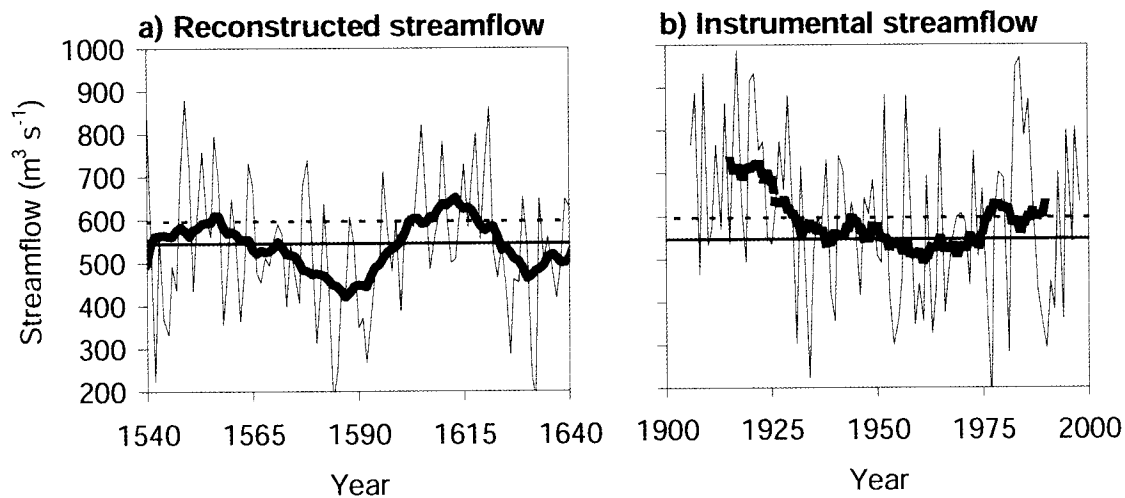
Figure 2. The “late sixteenth century megadrought” as recorded in a tree-ring reconstruction of mean annual streamflow of the Colorado River at Lees Ferry (left), and naturalized annual streamflow record from 1906 to 1998 (right). Thick lines represent the 20-year moving averages of both time series. The solid horizontal lines represent the long-term mean of the streamflow reconstruction, and the dashed lines represent the mean of the instrumental records.
