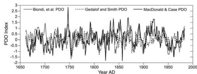
Figure 3. Comparison of our PDO reconstruction with the Biondi et al. [2001] and Gedalof and Smith [2001] reconstructions for the common period of AD 1661–1983.
