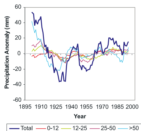
Figure 3. Time series of 13-yr moving average annual precipitation for 9-state western U.S. region. The 13-yr moving average values are plotted at the mid-point of the window. Time series are plotted for total annual precipitation and precipitation for 5-day periods occurring in one of 4 different categories: 0–12 mm, 12–25 mm, 25–50 mm, and >50 mm. Precipitation values are expressed as departures from normal.
