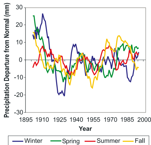
Figure 4. Time series of 13-yr moving average precipitation for the four seasons in the 9-state western region, expressed as a departure from normal.
