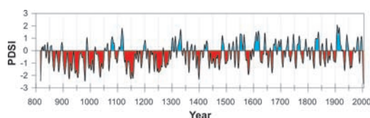
Figure 2. Regional reconstruction of the PDSI, AD 818–2003, smoothed with a 10-year spline. Red shading indicates negative values and dry years, and blue indicates positive values and wet years.
