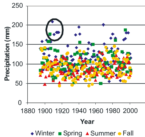
Figure 5. Seasonal precipitation (mm) averaged for the 9-state western U.S. region. Black oval highlights cluster of high values during the pluvial.
