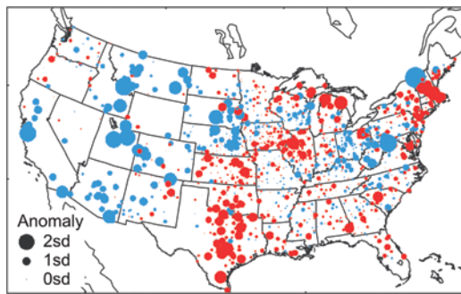
Figure 1. Annual standardized precipitation anomalies averaged for the period 1905–1917 for stations with at least 50 years of precipitation data and at least 10 years during 1905–1917. This includes 1284 U.S. stations with 136 stations in the nine-state pluvial region. Blue (red) circles indicate positive (negative) anomalies.
