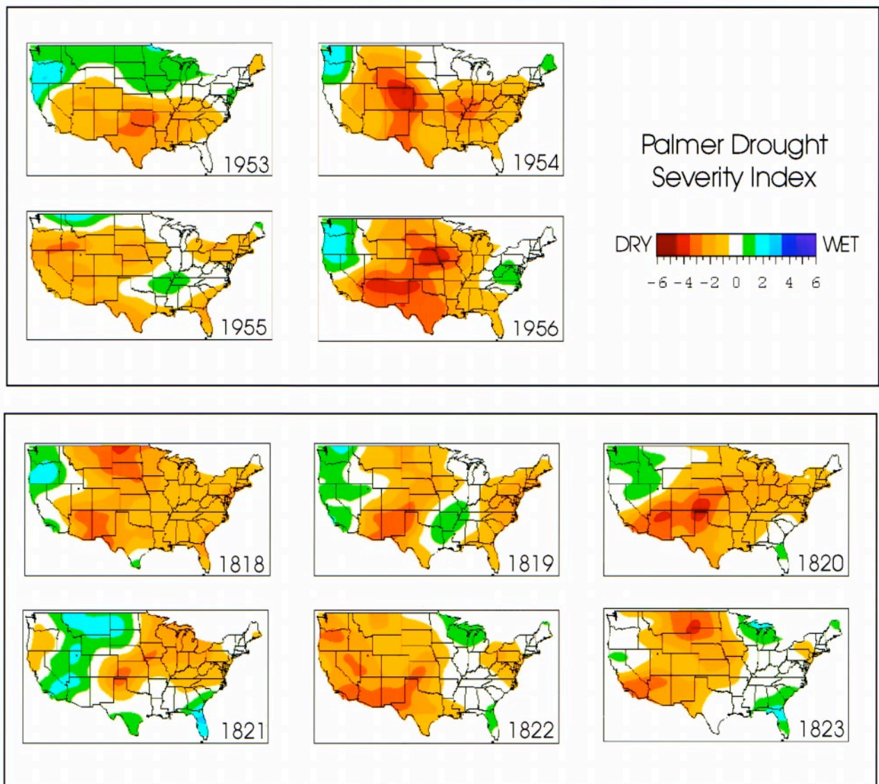
FIG. 7. Comparison of duration and extent of two severe droughts, the 1950s drought (top) and the drought centered on 1820 (bottom), both reconstructed from tree-ring chronologies (Cook et al. 1996; Cook et al. 1998).
