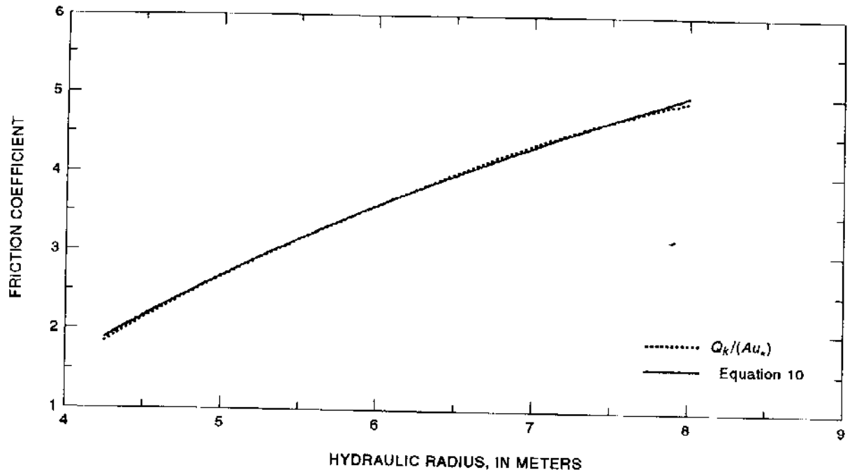
Figure 6. Relation between the hydraulic radius and the friction coefficient, \beta , calculated using equation 9 ( \beta=Q_k/(Au_s) ) in which cross-sectional area ( A ) is taken from equation 8 and using equation 10.
