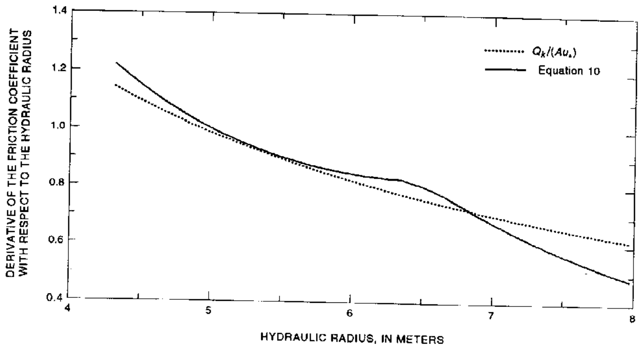
Figure 7. The derivative of the friction coefficient, \beta , with respect to the hydraulic radius plotted against the hydraulic radius.
