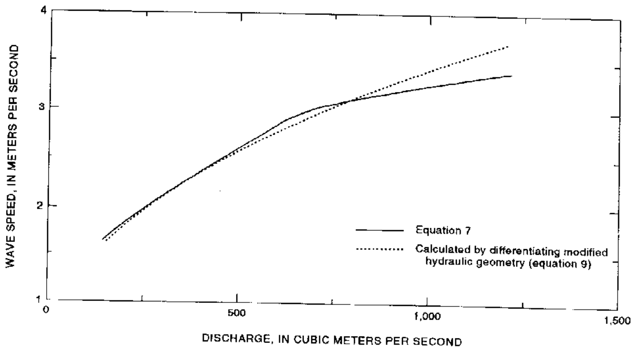
Figure 5. Wave speeds calculated with equation 7 and by differentiating discharge ( Q ) with respect to cross-sectional area ( A ) in equation 9.
