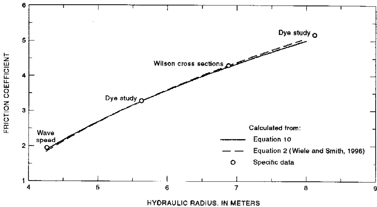
Figure 4. Relation between friction coefficient, \beta , and the hydraulic radius. Cross sections are from Wilson (1986).
