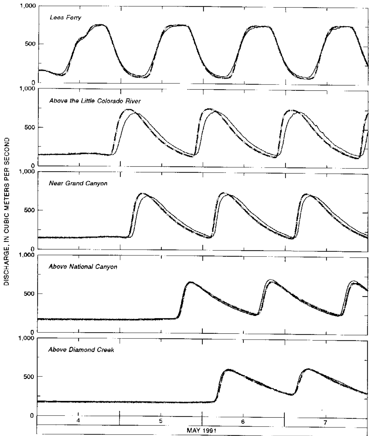
Figure 11. Hydrographs calculated with original (dashed lines) and modified (grey lines) models and hydrographs determined from stage records and the stage-discharge relations (solid lines) for research flow D at streamflow-gaging stations, Colorado River at Lees Ferry, Colorado River above the Little Colorado River near Desert View (RM 61), Colorado River near Grand Canyon (RM 88), Colorado River above National Canyon near Supai (RM 166), and Colorado River above Diamond Creek near Peach Springs (RM 225). The hydrographs are positioned to show the rise of the first wave following the steady flow.
