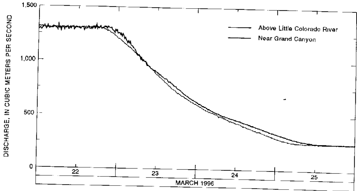
Figure 8. Hydrographs determined from stage records and stage-discharge relations at streamflow-gaging stations, Colorado River above the Little Colorado River near Desert View and Colorado River near Grand Canyon, for the receding limb of the controlled flood.
