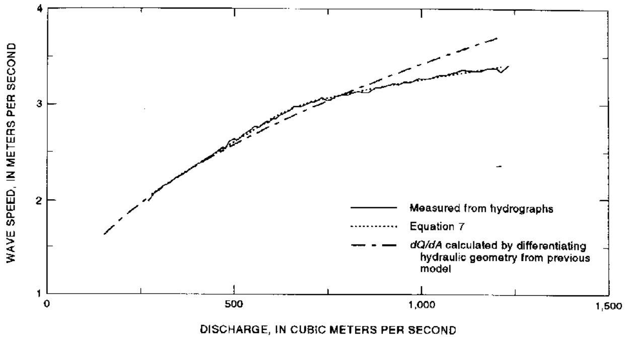
Figure 3. Wave speed calculated from the hydrographs from the streamflow-gaging stations, Colorado River at Lees Ferry and Colorado River above Diamond Creek near Peach Springs, calculated with equation 7, and calculated by differentiating the steady-flow discharge as a function of area calculated from the hydraulic geometry used in the original model.
