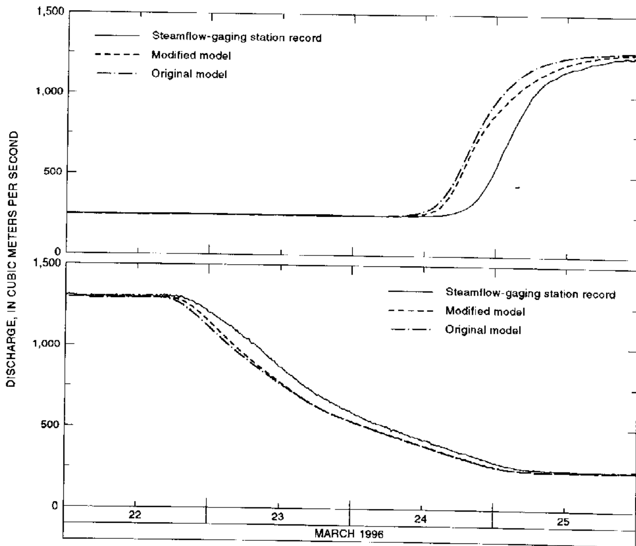
Figure 12. Hydrographs calculated with original and modified models and hydrographs determined from stage records and the stage-discharge relations for the rising (top) and falling (bottom) limbs of the controlled flood at streamflow-gaging station, Colorado River above Little Colorado River near Desert View.
