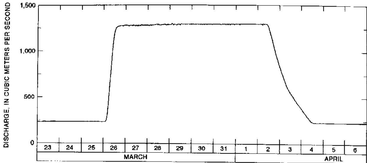
Figure 2. Hydrograph for the controlled flood released from Glen Canyon Dam, March–April 1996.
