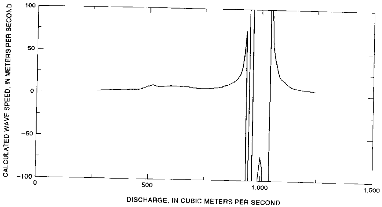
Figure 9. Wave speeds calculated from the hydrographs shown in figure 8. The long time of the falling limb makes calculation of wave speeds sensitive to the stage-discharge relations if the gaging stations are too close together.
