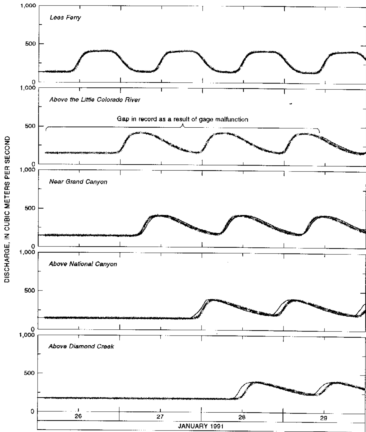
Figure 10. Hydrographs calculated with original (dashed lines) and modified (grey lines) models and hydrographs determined from stage records and the stage-discharge relations (solid lines) for research flow B at streamflow-gaging stations, Colorado River at Lees Ferry, Colorado River above the Little Colorado River near Desert View (RM 61), Colorado River near Grand Canyon (RM 88), Colorado River above National Canyon near Supai (RM 166), and Colorado River above Diamond Creek near Peach Springs (RM 225). The hydrographs are positioned to show the rise of the first wave following the steady flow with the exception of Colorado River, above the Little Colorado River near Desert View where the streamflow record is incomplete.
