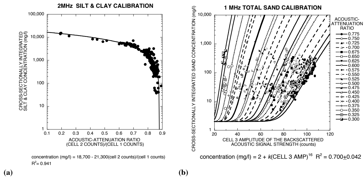
Figure 4. (a) Example of the relation between acoustic attenuation at 2 MHz (expressed as a ratio in counts between cells) and silt and clay concentration. (b) Example of the relations between the amplitude of the acoustic signal strength measured by the 1 MHz EZQ and total sand concentration for small ranges in the acoustic-attenuation ratio arising from silt and clay. The coefficient k relates the sand-calibration curves as a function of the acoustic attenuation ratio, i.e., silt and clay concentration (relation has R^2 = 0.986 ).
