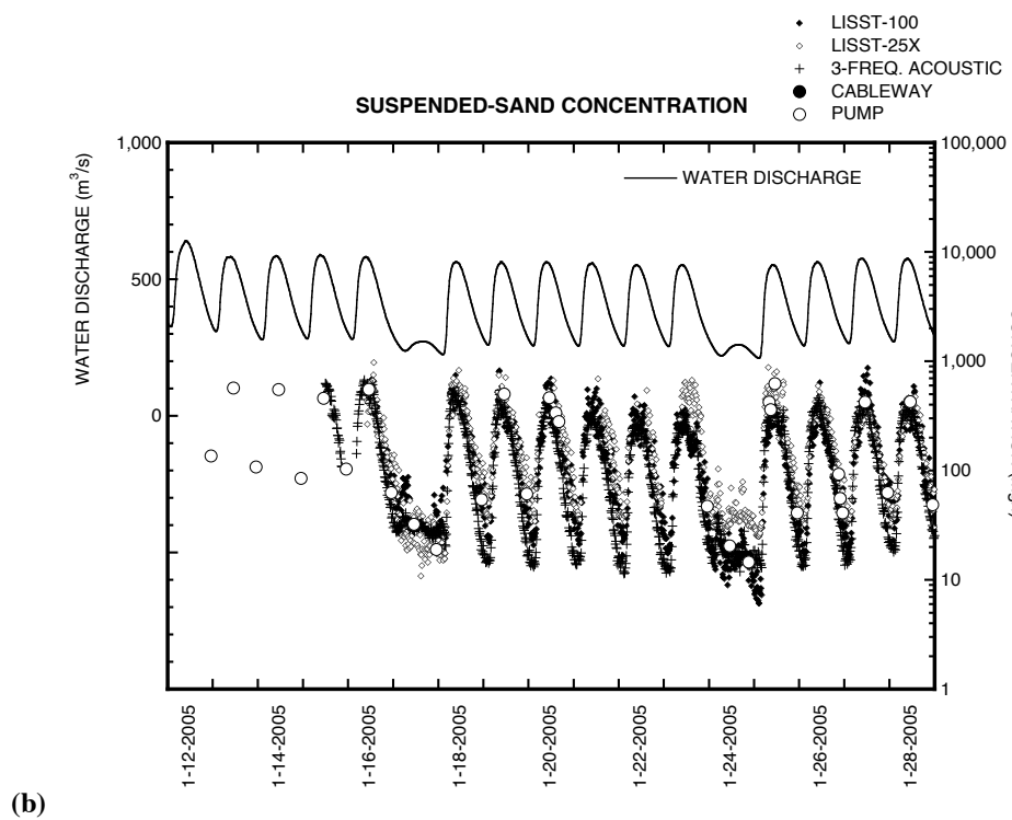
Figure 5. Examples of the high-resolution laser-acoustic suspended-sediment data from beyond the period of calibration. No EDI measurements were made from the cableway during this 17-day period. Silt and clay concentrations were too high during the first 3 1/2 days of this period to get LISST or acoustic measurements of suspended-sand concentration or median grain size. (a) Silt and clay concentration, (b) Sand concentration, (c) Suspended-sand median grain size ( D_{50} ); on next page.
