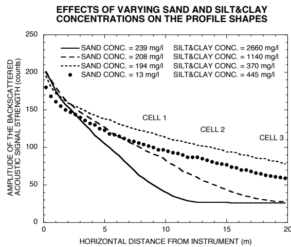
Figure 3. Effects of varying sediment concentration on acoustic profiles collected with the 1 MHz EZQ. Changes in silt and clay concentration mainly result in changes in the slope of the profile; changes in sand concentration mainly result in upward or downward shifts in the profile without changing the slope.
