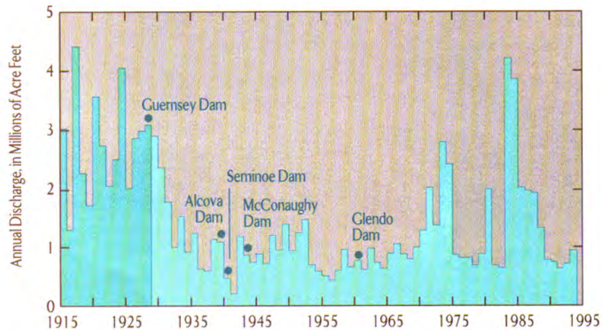
Annual flow volumes for the Platte River at Overton, Nebraska. Five dams built since 1909 provide flow regulation for irrigation of farmland in Wyoming, Nebraska, and eastern Colorado.
