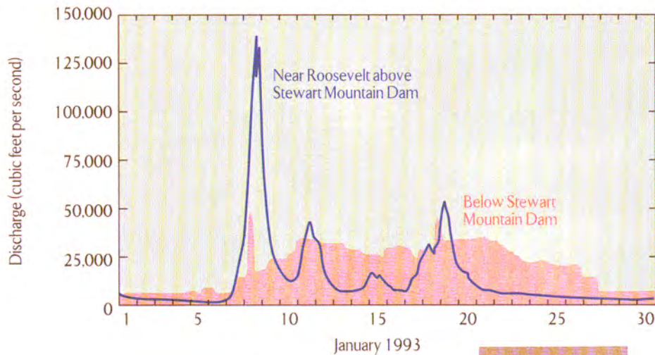
Hydrograph of the Salt River for January 1993. Peak discharge reached 143,000 ft 3 /s on January 9 above Roosevelt Dam. Releases from Stewart Mountain Dam, the farthest downstream of four dams on the Salt, are dampened and protracted compared to the inflow to Roosevelt Lake.
