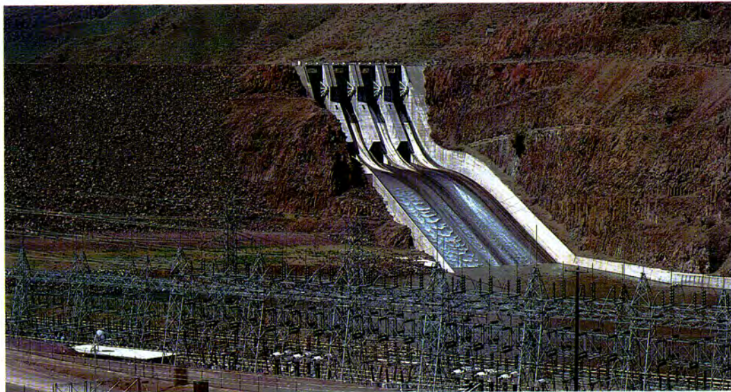
Brownlee Dam on the Snake River
