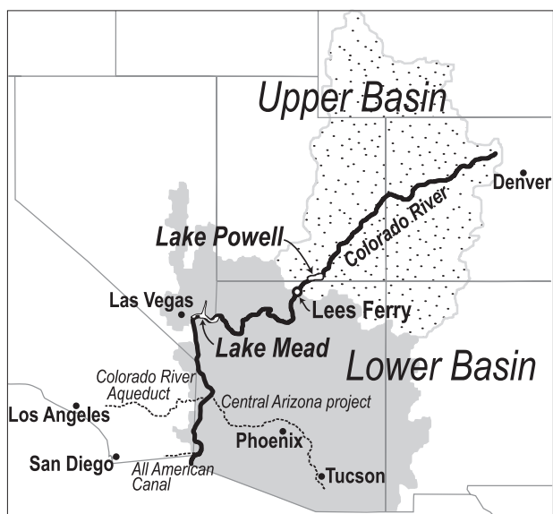
Figure 1. Overview of the region of interest ( 31.2^{\circ} – 43.7^{\circ} N, 104.0^{\circ} – 120.3^{\circ} W), which is historically separated into the “upper basin” (dots) and “lower basin” (gray). Colorado River flow from the upper to lower basins is measured at Lees Ferry.
