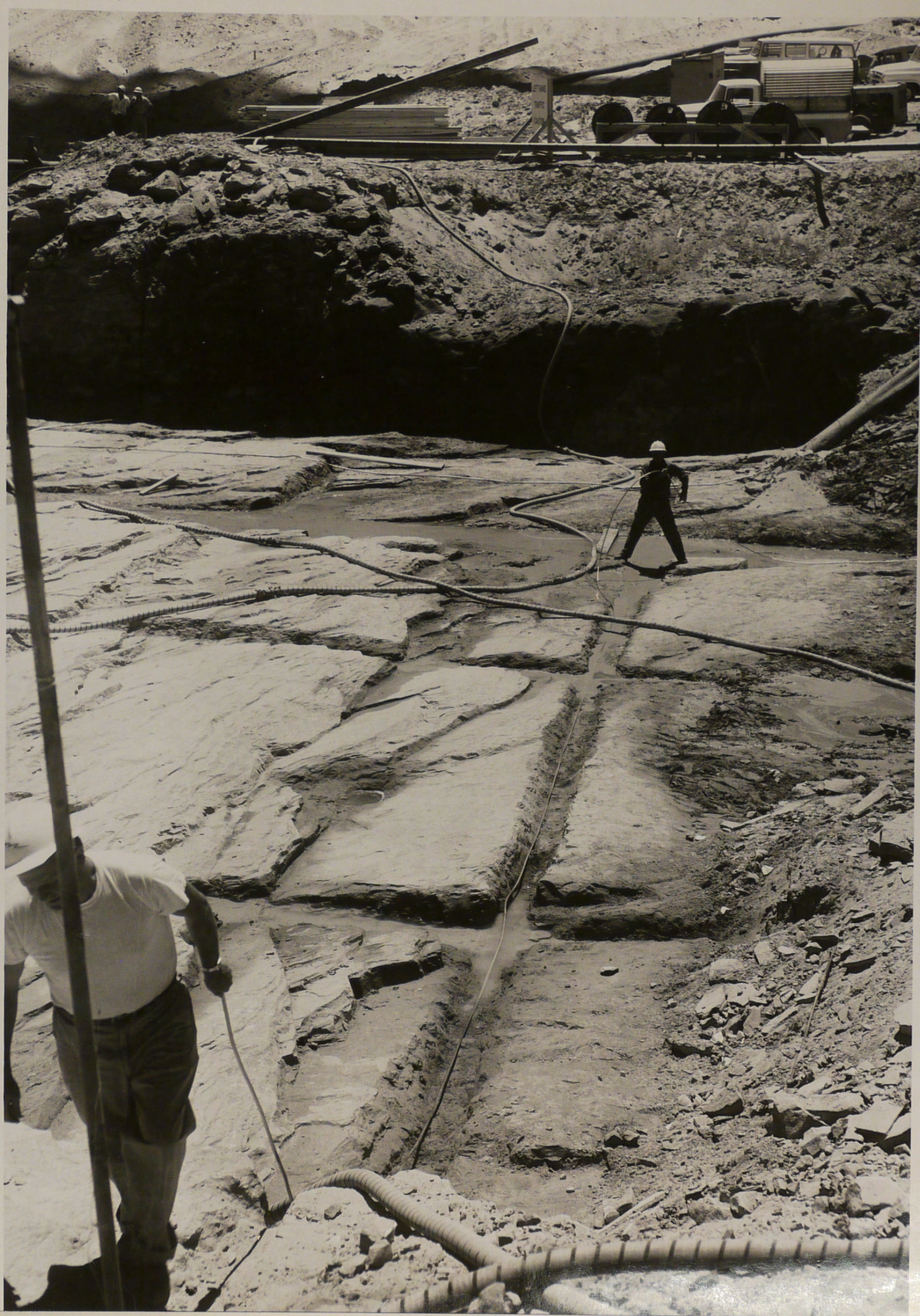
P 557-420-04892 Glen Canyon Unit--C.R.S.P. Laying ground mat in Unit Bay 3. Contractor: Merritt-Chapman and Scott Corporation. Contract No. 14-06-D-2403, Specs. No. DC-4825. 5-26-60 A. E. Turner
