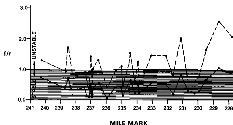
Fig. 9. The stability ratio calculated by the method shown in Figure 4 and field data from the Canyon of Lodore. Dashed line shows predam conditions; solid line shows postdam conditions. Mile marks as surveyed by Herron [1917], also found in the works by Evans and Belknap [1973] and Hayes and Simmons [1973].
