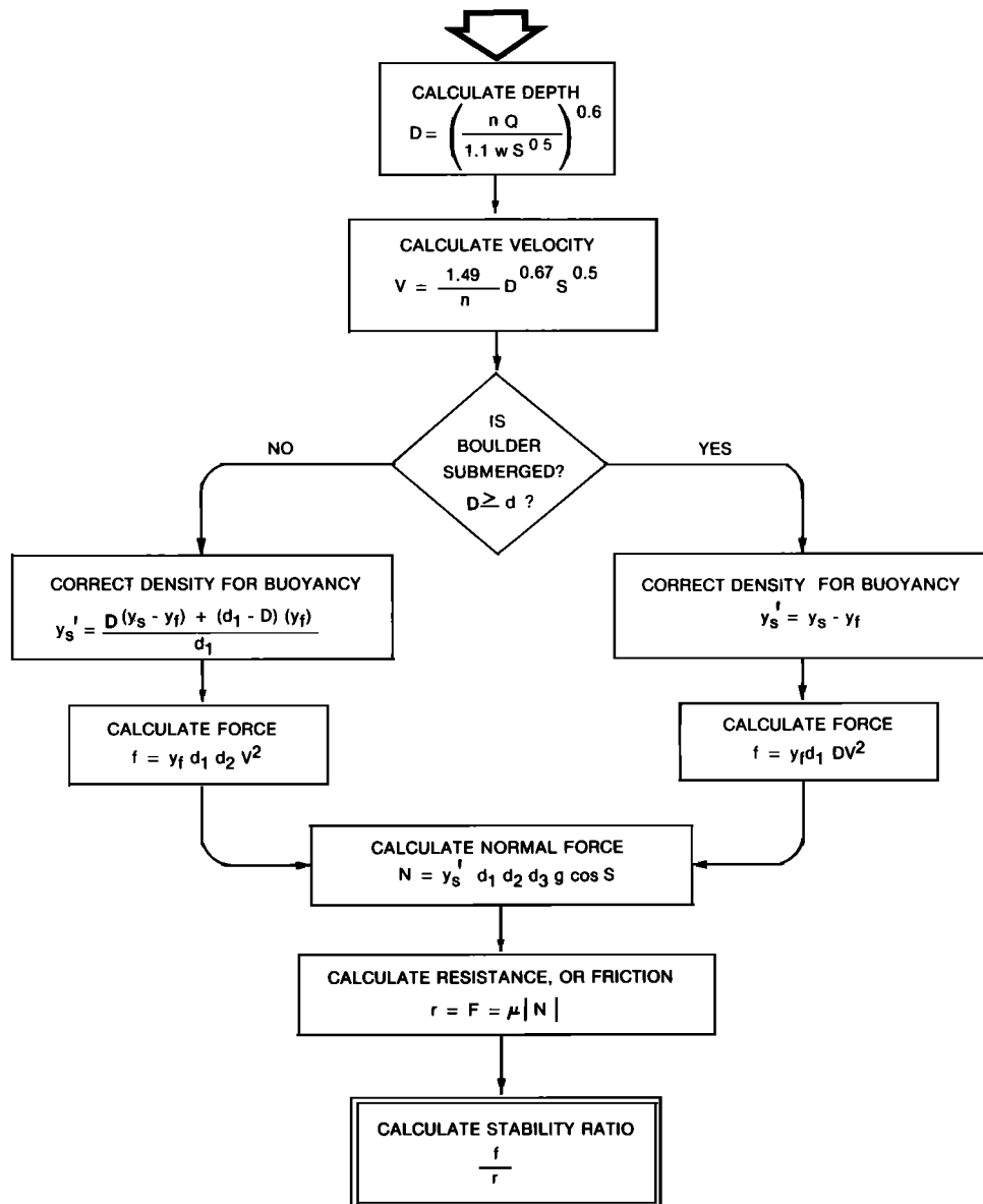
Fig. 4. Method for calculating the stability of the largest boulder in rapids. Symbols with dimensions: D is the depth of flow (in meters); d_1, d_2, \dots are the primary dimensions of the boulder (in meters); F is the friction (in newtons); f is the force of flowing water against upstream face of the boulder (in newtons); g is the acceleration of gravity (in meters per second per second); \mu is the coefficient of friction (dimensionless); N is the normal force (in newtons); n is the Manning roughness coefficient (dimensionless); Q is the discharge (in cubic meters per second); S is the gradient (dimensionless); w is the channel width (in meters); y_f is the density of the fluid (in kilograms per cubic meter); y_s is the density of the boulder and y'_s is the density of the boulder corrected for buoyancy (in kilograms per cubic meter).
