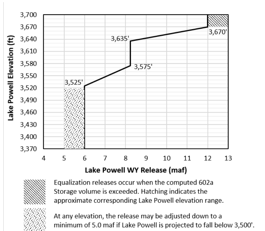
Figure A-6 Lake Powell Operations Diagram, Representative Preferred Alternative
