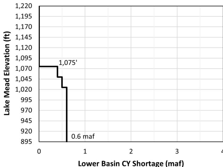
Figure A-7 Shortage Guidelines to Reduce Deliveries from Lake Mead, No Action Alternative
