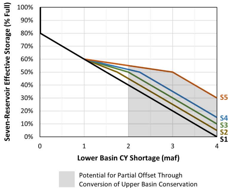
Figure A-10 Shortage Guidelines to Reduce Deliveries from Lake Mead, Maximum Operational Flexibility Alternative
