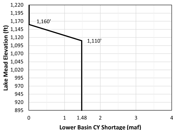
Figure A-8 Shortage Guidelines to Reduce Deliveries from Lake Mead, Basic Coordination Alternative
