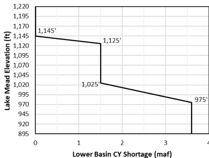
Figure A-12 Shortage Guidelines to Reduce Deliveries from Lake Mead, Representative Preferred Alternative
