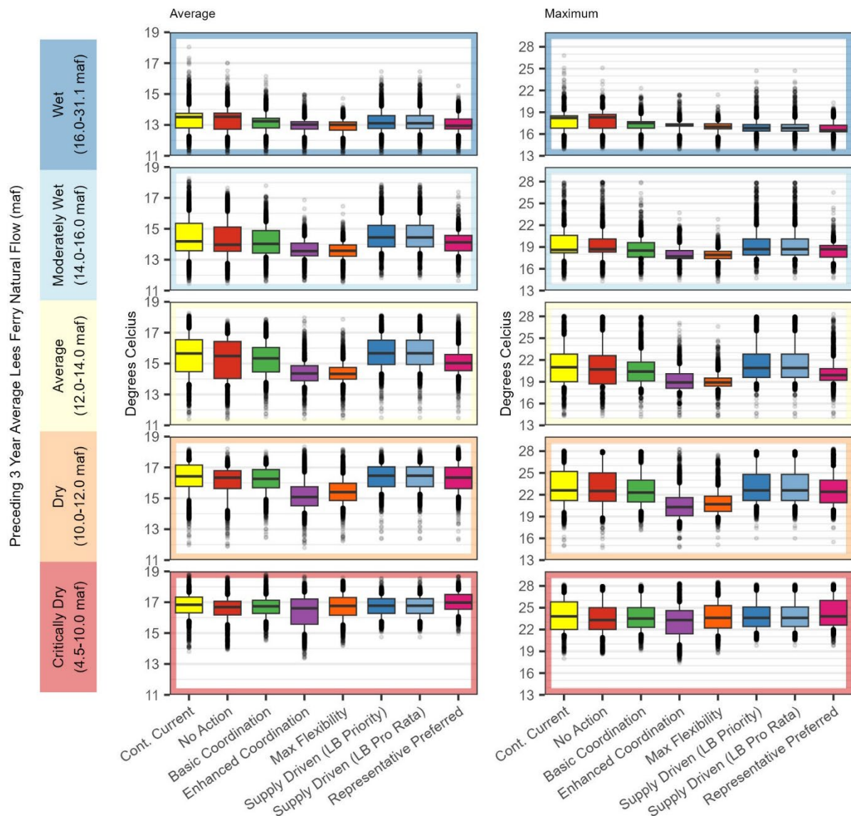
Figure TA 6-10 Average* and Maximum** Colorado River Temperature at Pearce Ferry
