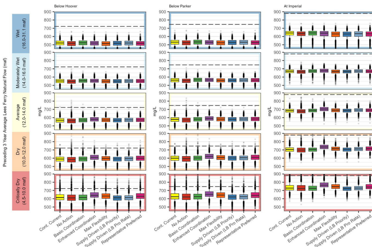
Figure TA 6-4 Annual Flow-Weighted Average Salinity Concentrations
