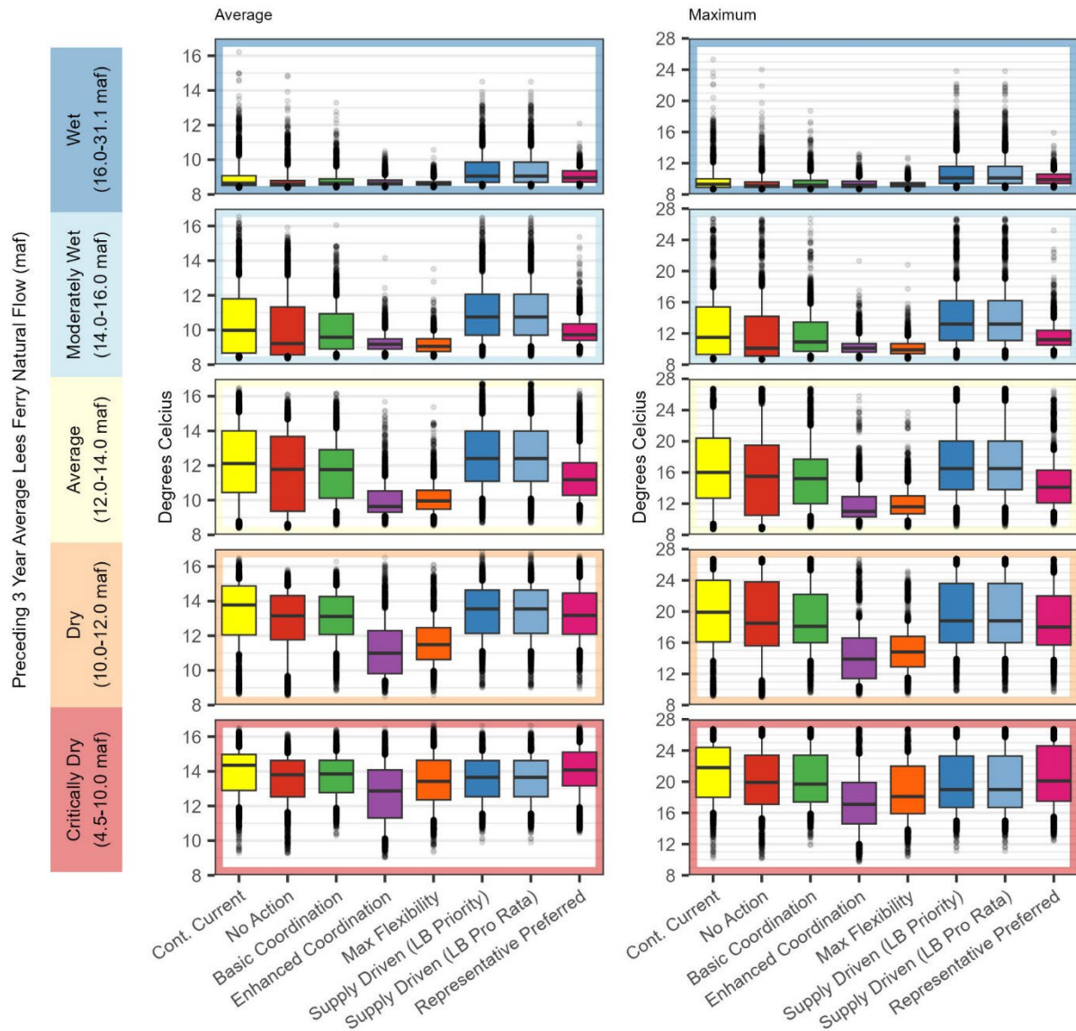
Figure TA 6-9 Average* and Maximum** Colorado River Temperature at Lees Ferry
