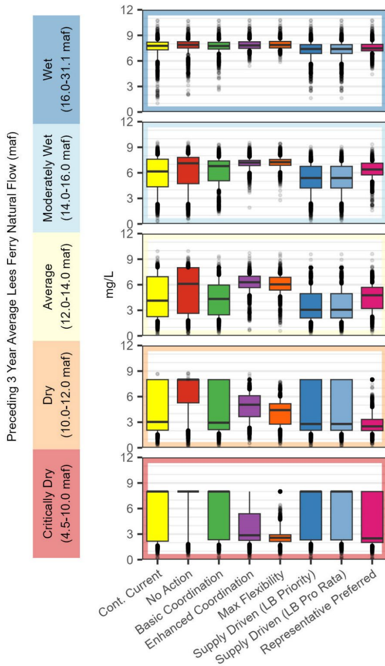
Figure TA 6-11 Minimum Annual Dissolved Oxygen Concentration Released from Glen Canyon Dam*
