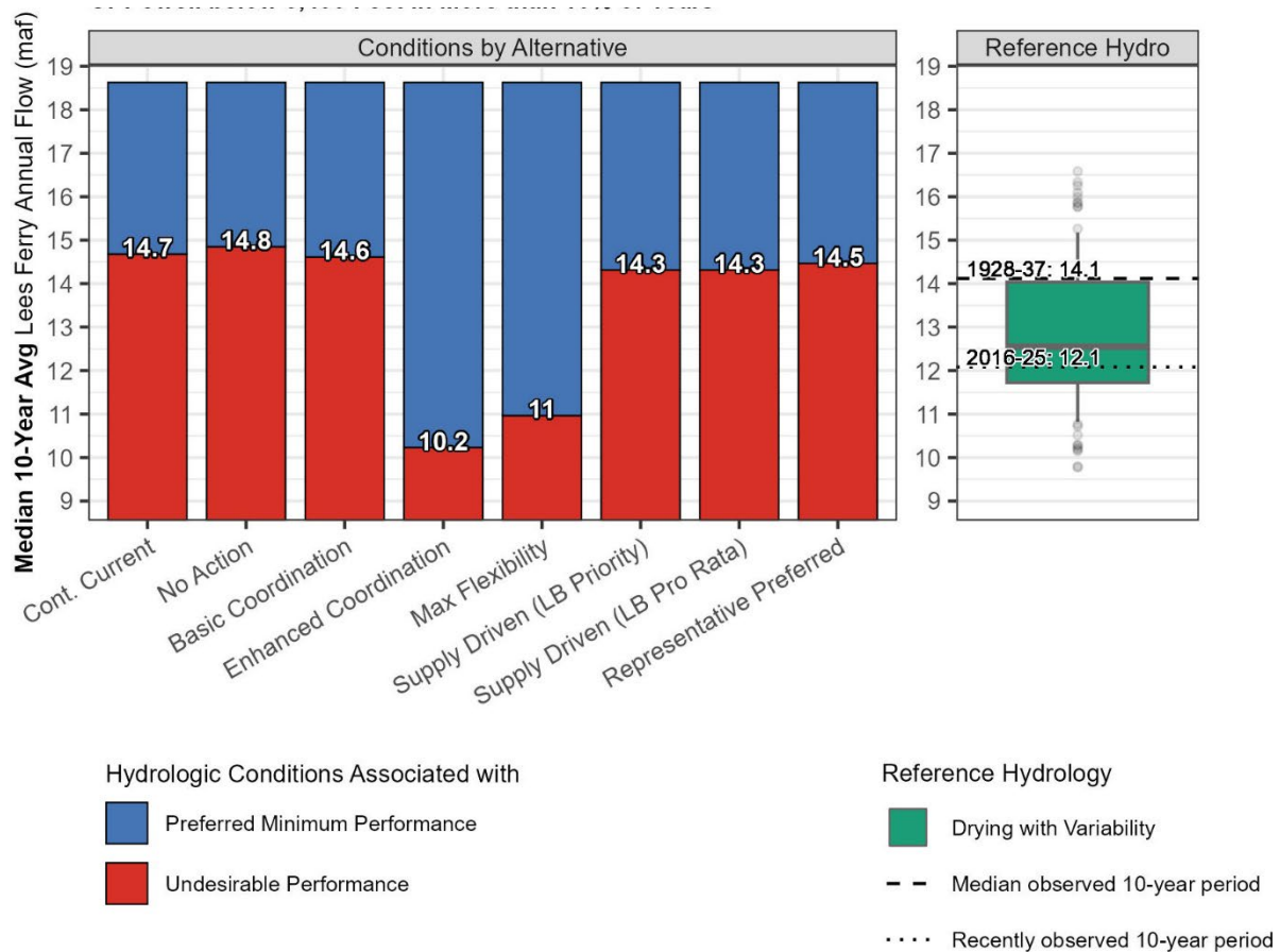
Figure TA 6-14 Lake Powell 3,490 and Dissolved Oxygen Concentration: Vulnerability. Conditions that Could Cause Dissolved Oxygen Concentration Less than 2 mg/L or Powell below 3,490 Feet in More than 10 percent of Years.
