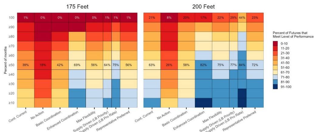
Figure TA 19-10 Monthly Height of Lake Mead Calcium Carbonate Ring 2027-2039: Robustness. Percentage of futures in which the height of the calcium carbonate ring at Lake Mead is less than the reference height in the percentage of months specified by each row
