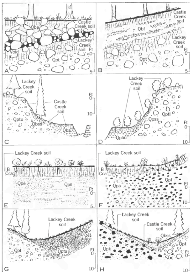
FIGURE 22.—Some stratigraphic relations of deposits of the Placer Creek formation.
