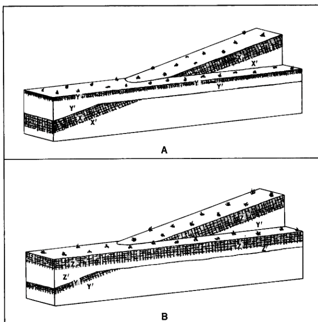
FIGURE 11.—Determination of the usefulness of relict soils as stratigraphic horizons.
