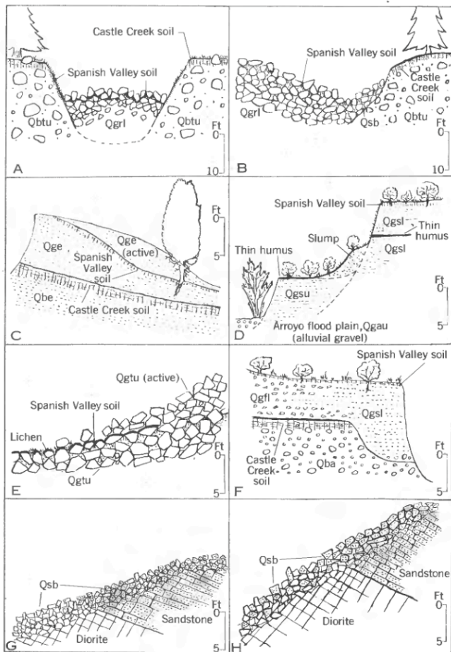
FIGURE 45.—Some stratigraphic relations of deposits of the Gold Basin formation.
