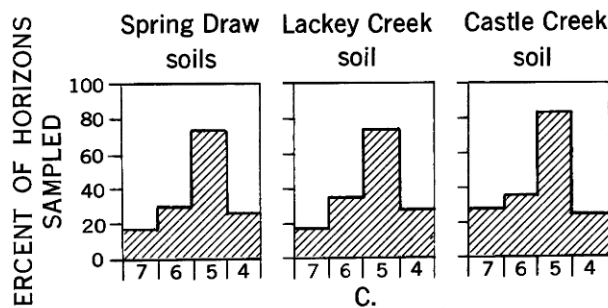
FIGURE 57.—Range in color properties of B horizon of soils of different geologic age in the La Sal Mountains, Utah. A, Range in hue of B horizon; B, range in chroma of B horizon; C, range in color value of B horizon.
