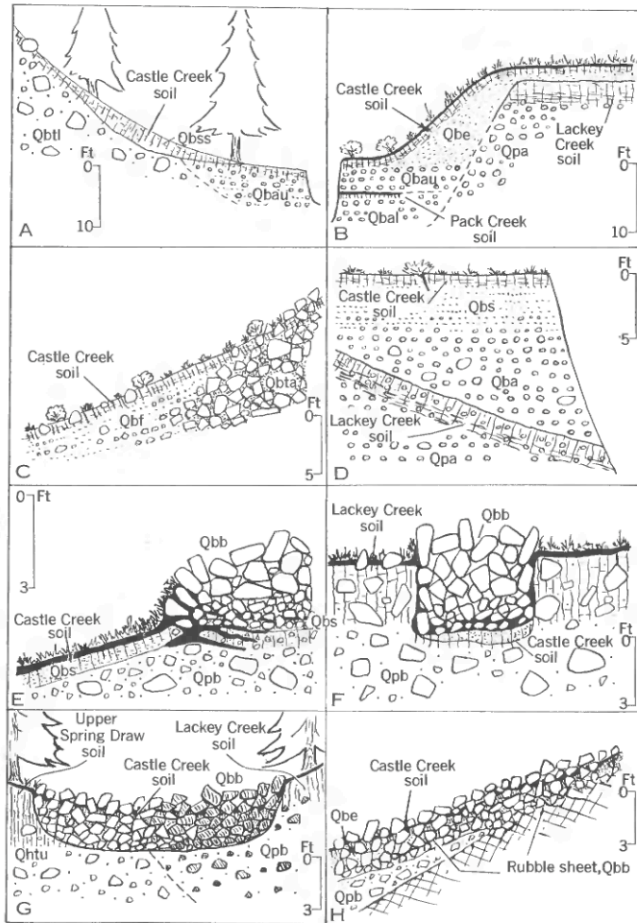
FIGURE 30.—Some stratigraphic relations of deposits of the Beaver Basin formation.
