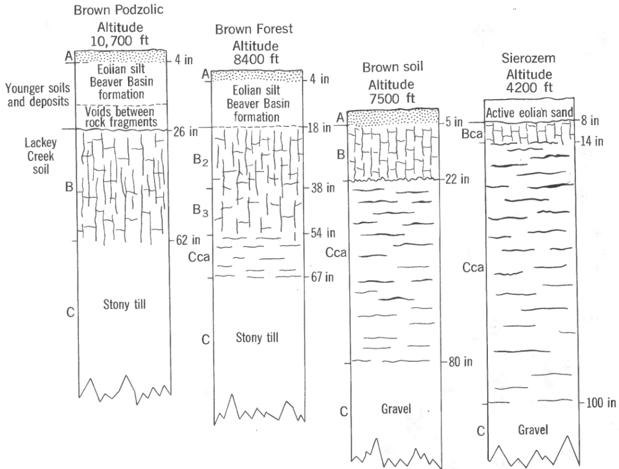
FIGURE 29.—Typical profiles of the four major facies of the Lackey Creek soil showing, diagrammatically, their general character and thickness on parent material composed chiefly of diorite.
