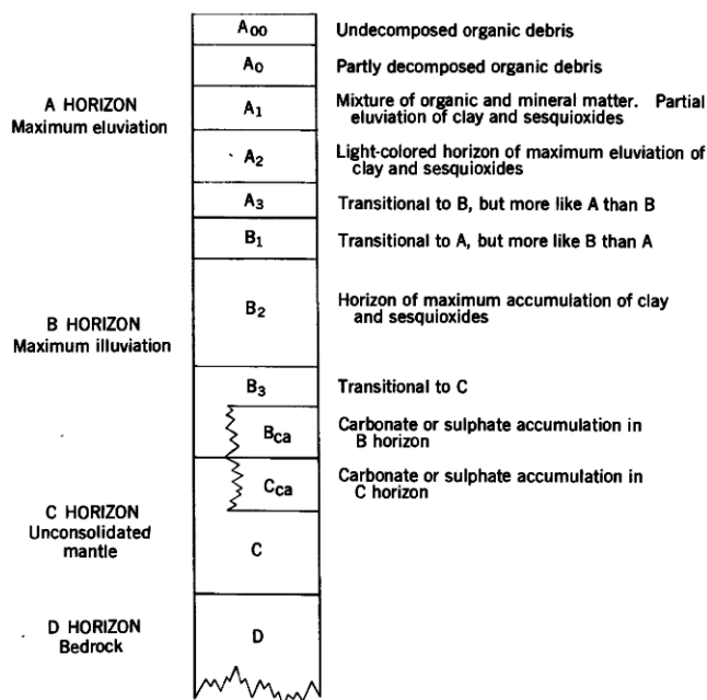
FIGURE 10.—Possible horizons in soil profiles.
