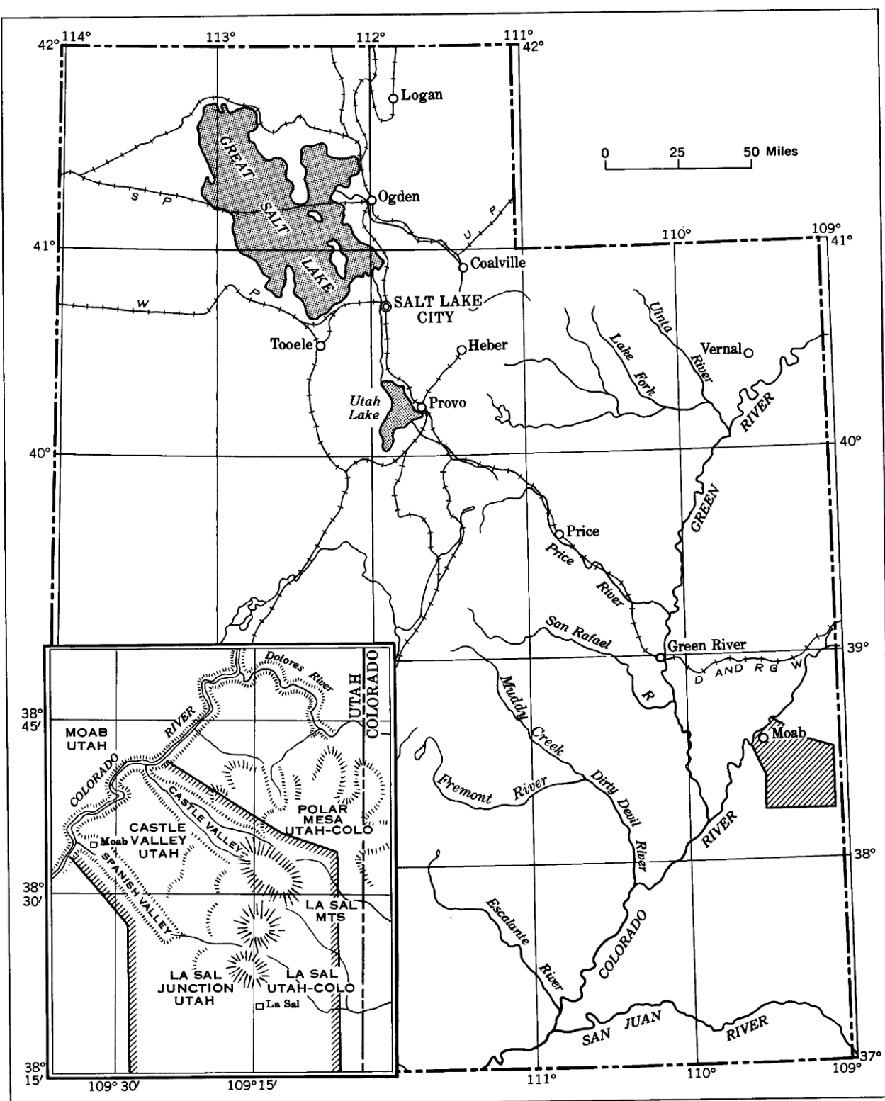
FIGURE 1.—Index map showing location of the La Sal Mountains in southeastern Utah.
