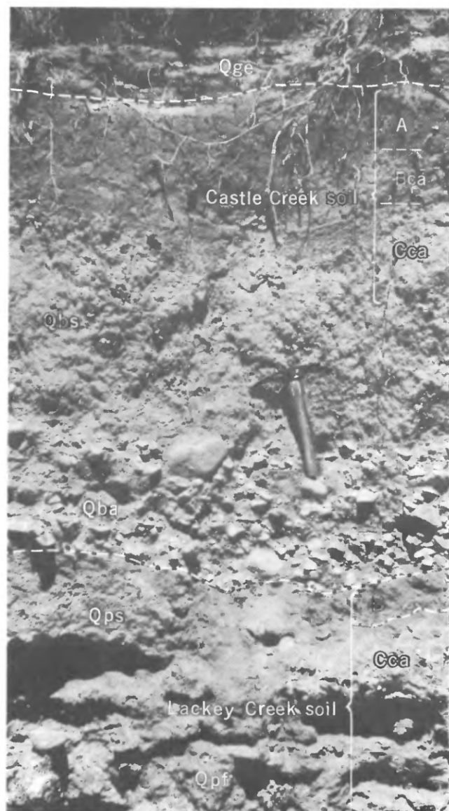
FIGURE 28.—Type locality of the Lackey Creek soil in the wall of Lackey Creek 2½ miles west of La Sal just downstream from the crossings of State Highway 46. The Brown soil facies of the strongly developed Lackey Creek soil is formed on alluvial silt ( Qps ) and fan gravel ( Qpf ) of the lower member of the Placer Creek formation, and is overlain disconformably by fan gravel ( Qba ) and alluvial silt ( Qbs ) of the Beaver Basin formation on which the moderately developed Castle Creek soil is formed. Recent eolian silt ( Qge ) overlies these deposits at the top of the section.
