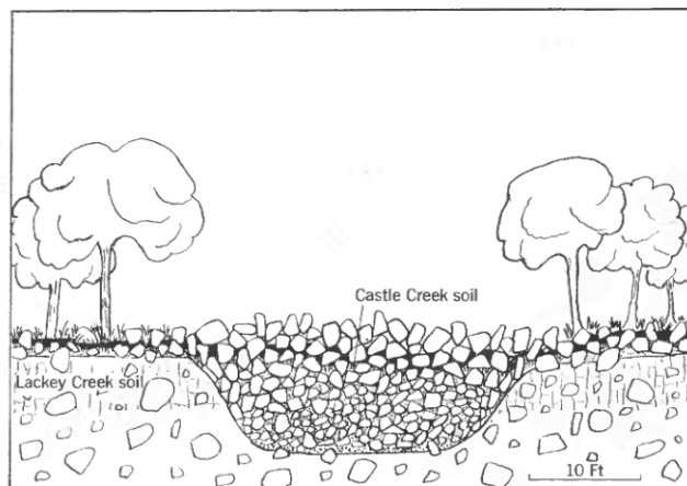
FIGURE 34.—Cross section of a rubble stream of the Beaver Basin formation developed on bouldery till of the Placer Creek formation along the road to Miners Basin at an altitude of 9,400 feet. The rubble stream truncates the profile of the Lackey Creek soil developed on the till. Some of the fine material, removed from the till during formation of the rubble stream, has settled at its base. Above, the interstices of the rubble were filled with eolian sand at some time after the rubble stream became stagnant. The sand is well sorted and composed almost wholly of quartz, in contrast to the poorly sorted and highly feldspathic character of the matrix of the till. The profile of the Castle Creek soil is formed on the eolian sand at a depth of from 2 to 4 feet below the surface of the rubble stream.
