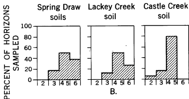
FIGURE 56.—Range in maximum thickness of B or Bca horizon with altitude in soils of different geologic age in the La Sal Mountains, Utah.
