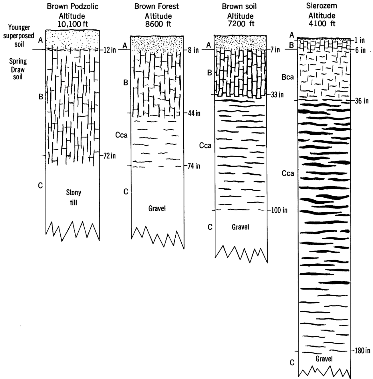
FIGURE 18.—Typical profiles of the four major facies of the Spring Draw soils, showing diagrammatically their general character and thickness.
