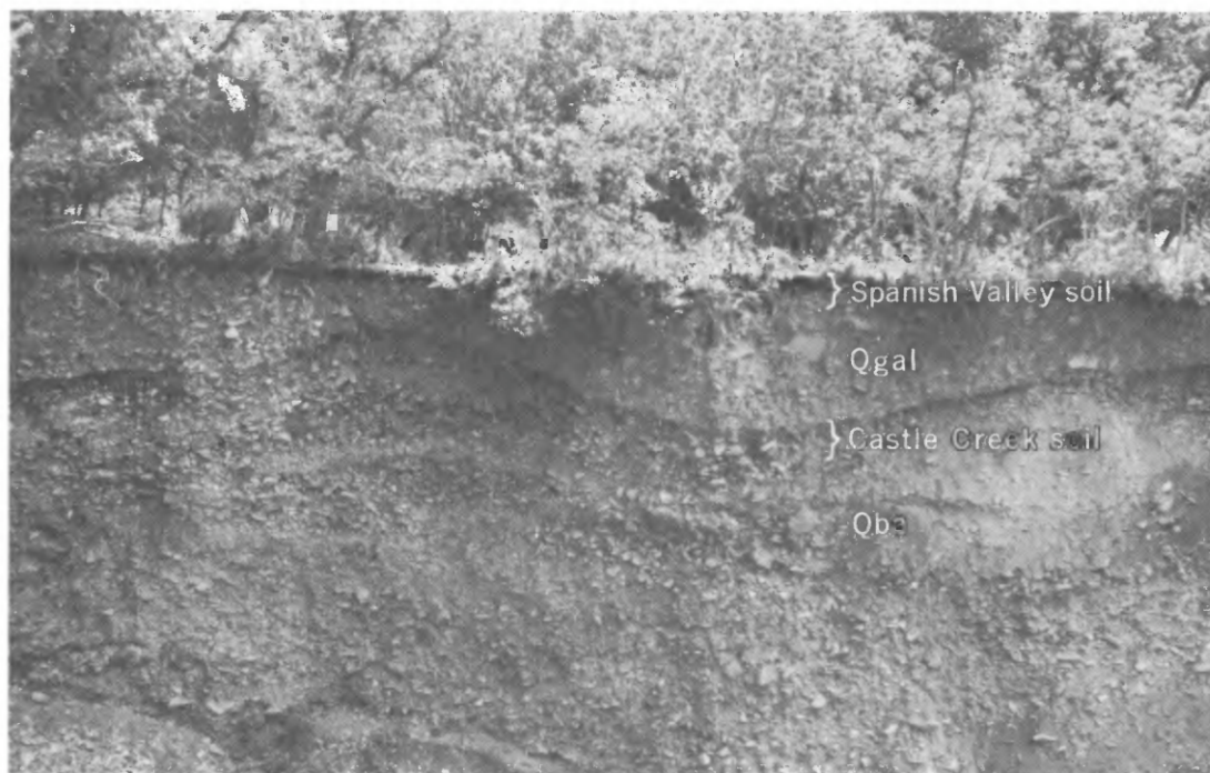
FIGURE 49.—Alluvial gravel of the lower member of the Gold Basin formation ( Qgal ), on which the Spanish Valley soil is developed, overlapping the Castle Creek soil on alluvial gravel ( Qba ) of the Beaver Basin formation. Exposure is along the upper sector of Pack Creek at an altitude of 9,100 feet.
