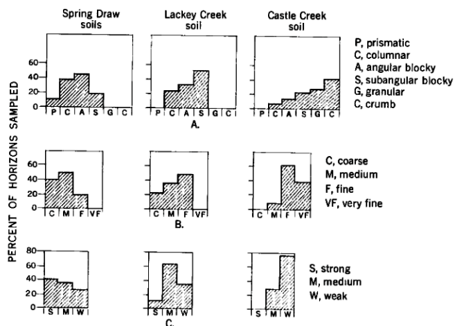
FIGURE 58.—Range in structural properties of B horizon of soils of different geologic age in the La Sal Mountains, Utah. A, Range in type of structure; B, range in class of structure; C, range in grade of structure.
