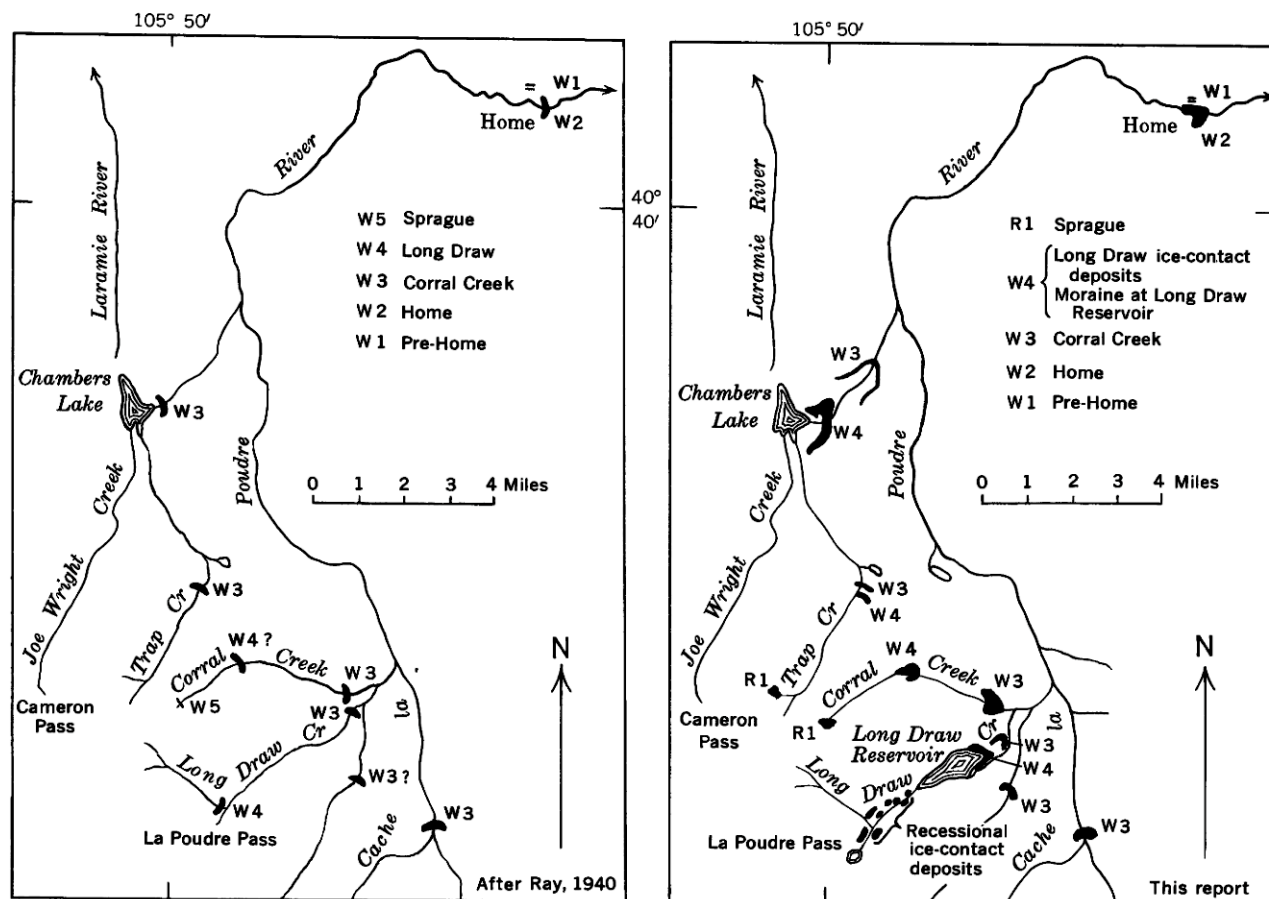
FIGURE 62.—Sketch maps comparing interpretations of moraines in the Cache la Poudre drainage system.
