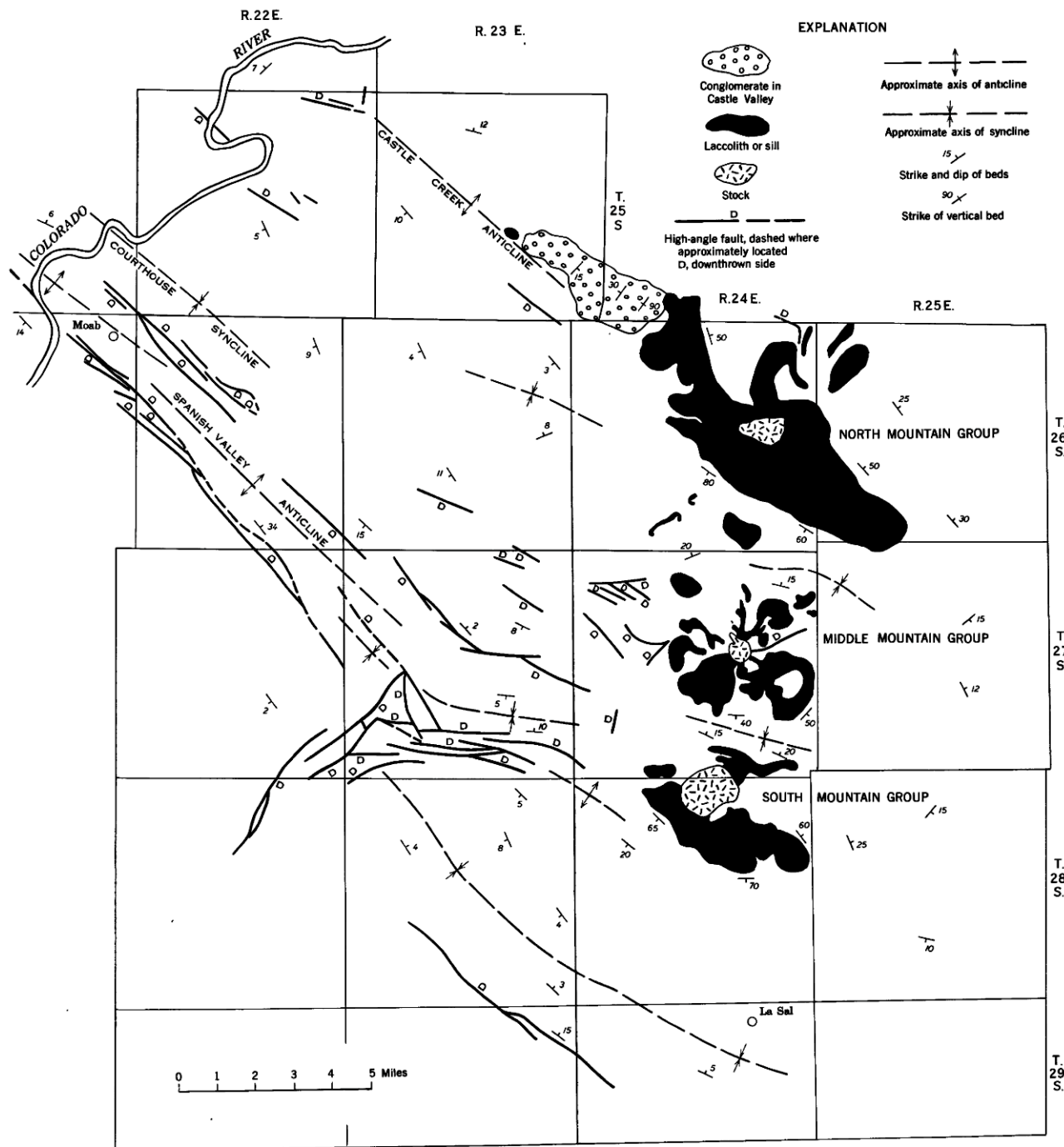
FIGURE 2.—Generalized map of the geologic structure in the vicinity of the La Sal Mountains (compiled after Baker, 1933, and Hunt, 1958).
