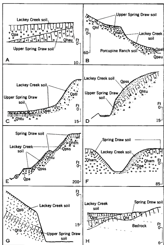
FIGURE 17.—Some geologic relations of the Spring Draw soils.
