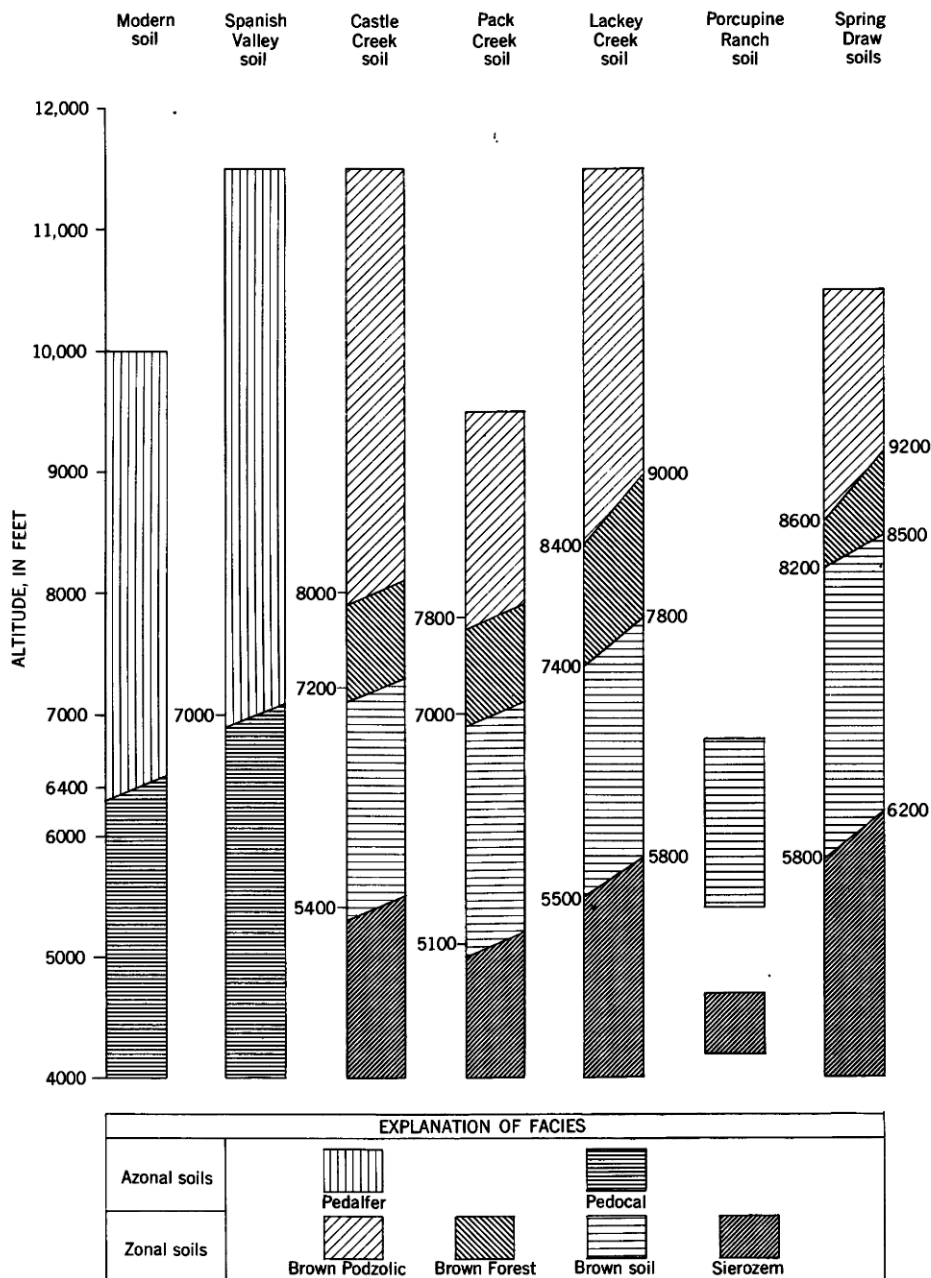
FIGURE 19.—Range in altitude of facies and facies changes of soils of different geologic age in the La Sal Mountains, Utah. Altitudes beside columns are average altitudes of facies changes.
