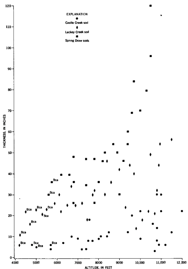
FIGURE 56.—Range in maximum thickness of B or Bca horizon with altitude in soils of different geologic age in the La Sal Mountains, Utah.
