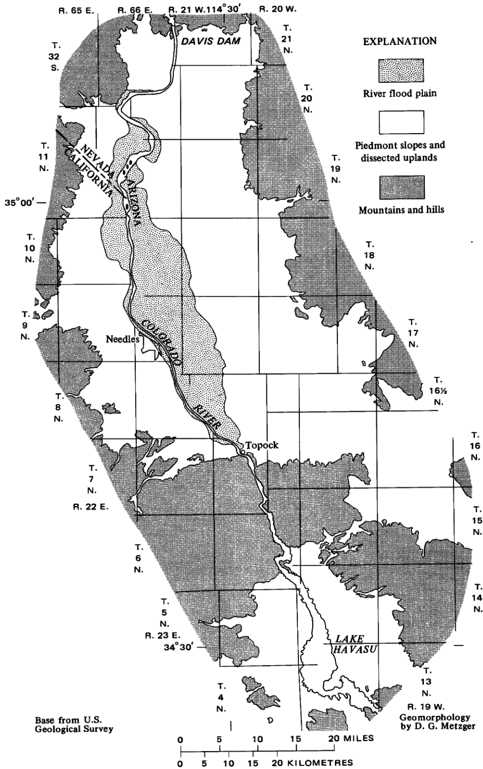
FIGURE 7.—Landforms in the Needles area.
