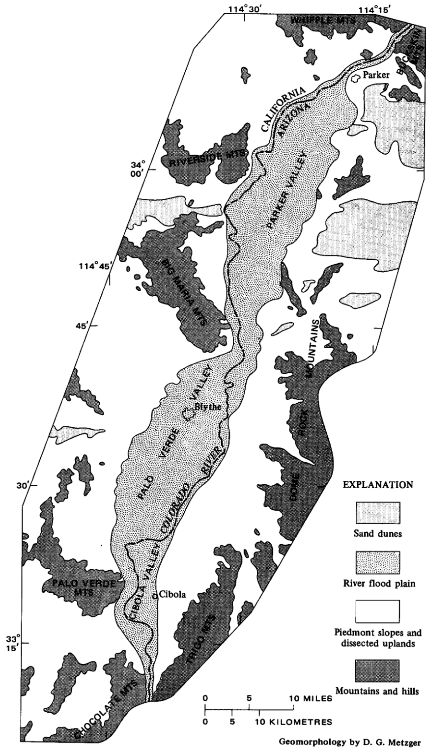
FIGURE 8.—Landforms in the Parker-Blythe-Cibola area.
