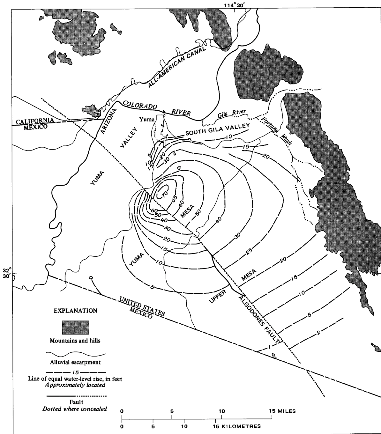
FIGURE 12.—Change in water level beneath Yuma Mesa, 1925-66
