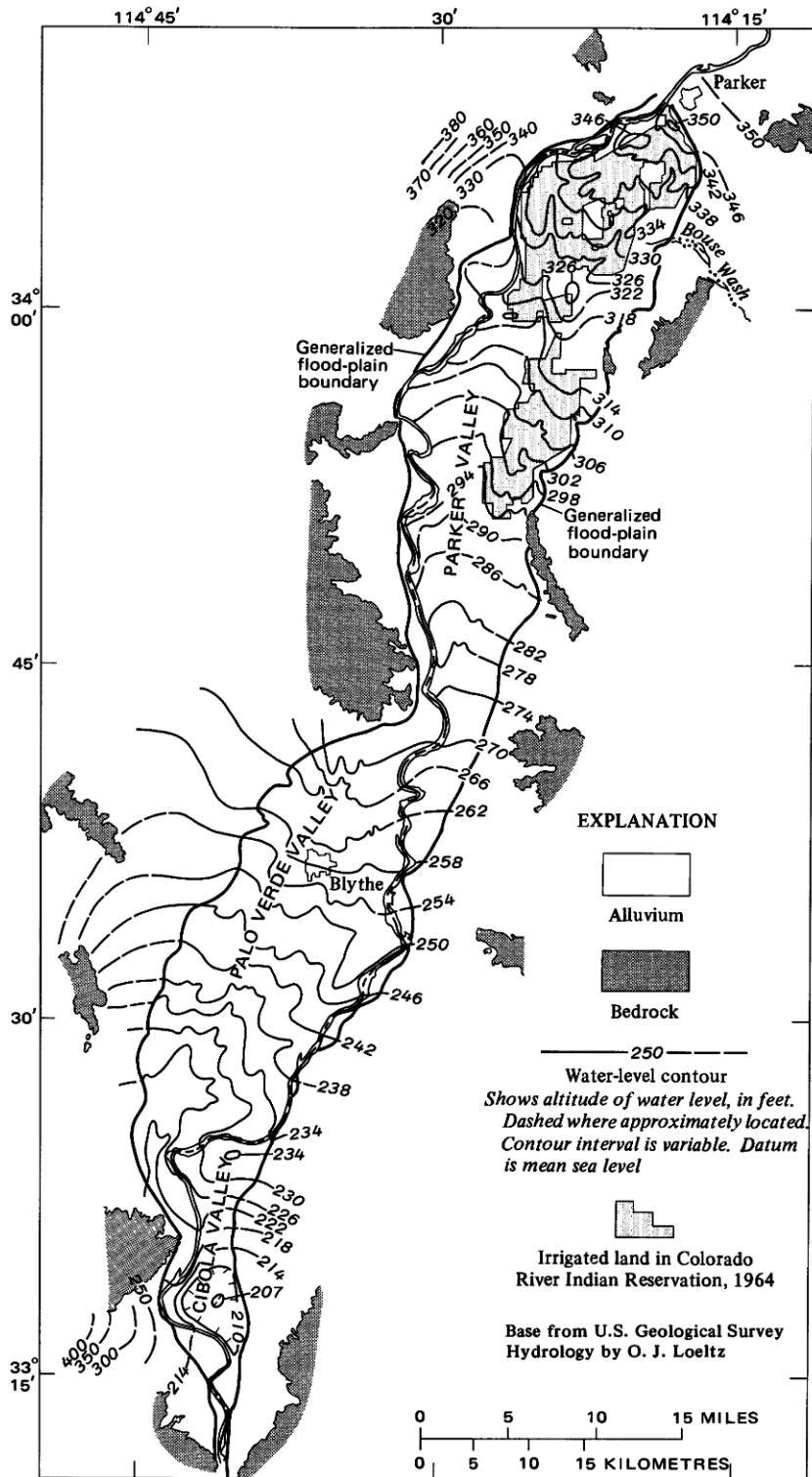
FIGURE 14.—Generalized water-level contours in Parker-Blythe-Cibola area, 1964.
