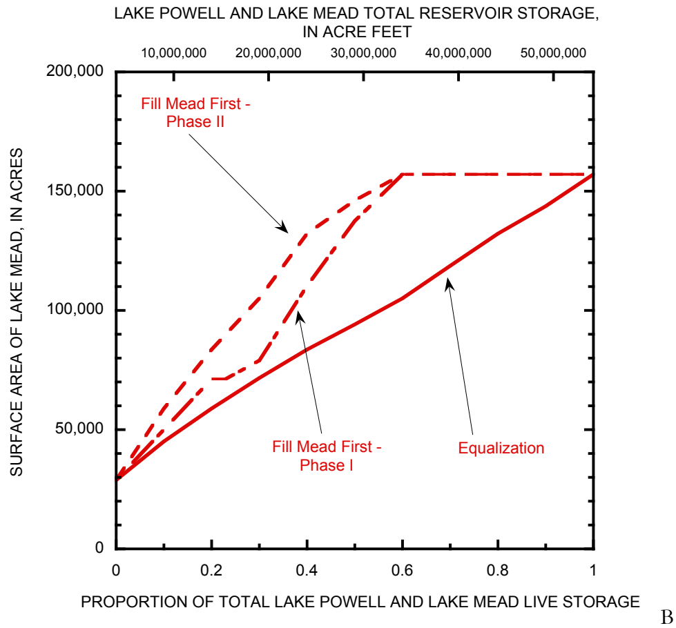
Figure 14. Graphs showing the surface area of Lake Powell (A) and Lake Mead (B) for the present equalization strategy and for the two phases of FMF. These data are based on the storage-to-surface area relations shown in Figure 7 multiplied by the scenarios shown in Figure 10.
