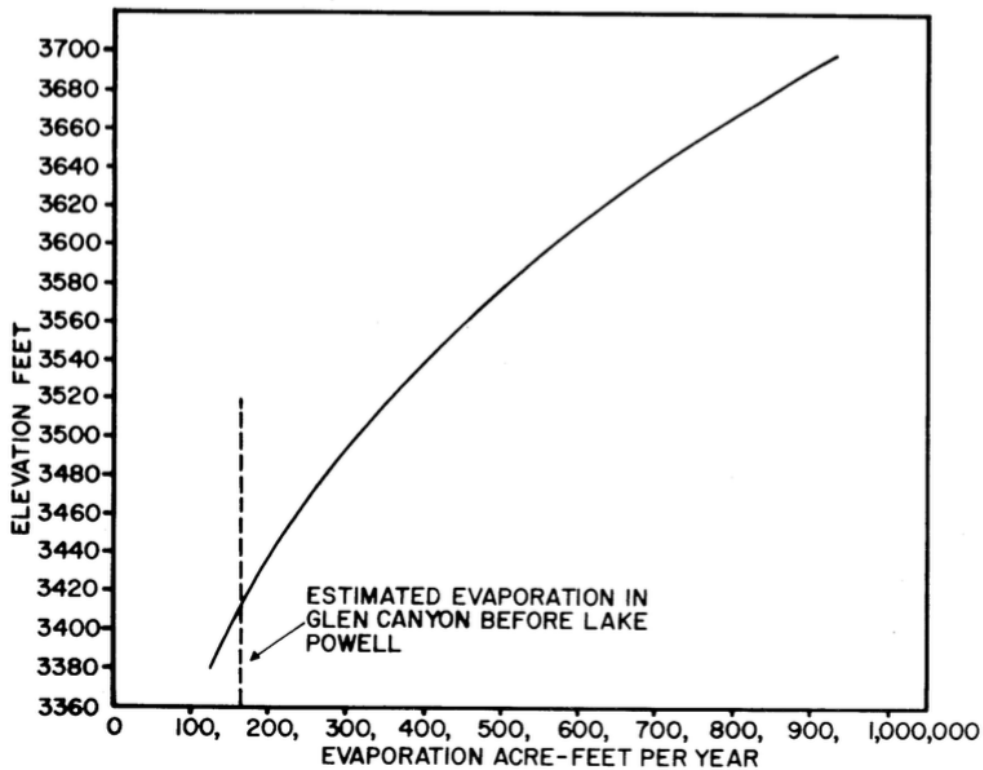
Figure 12. Graph showing the annual evaporation from Lake Powell as a function of reservoir elevation (from Jacoby et al., 1977, fig. 16).
