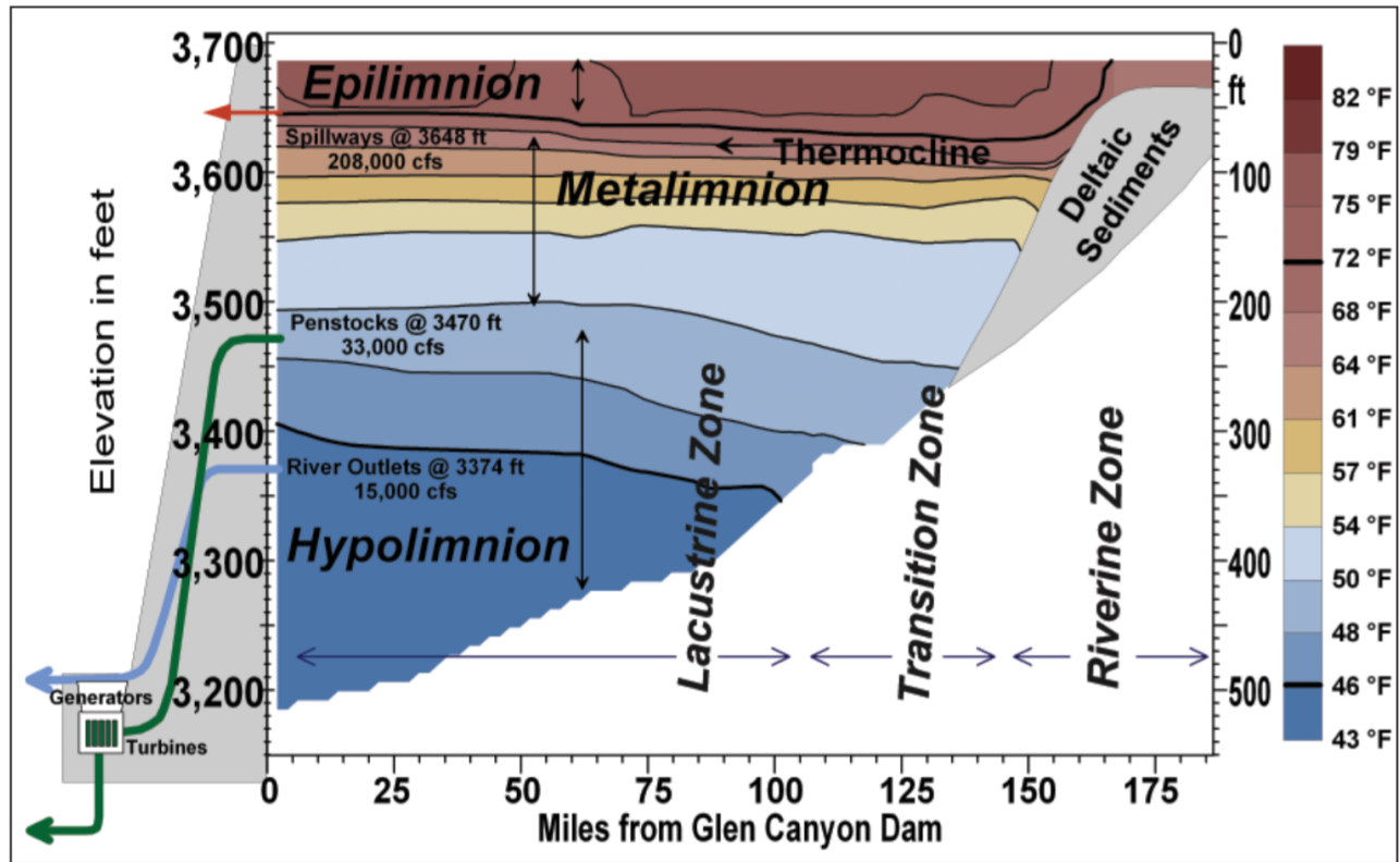
Figure 2. Diagram showing typical temperature stratification of Lake Powell at times when the reservoir is nearly full and showing the elevations of the three facilities through which water is released from Lake Powell to the downstream Colorado River. Also shown is the approximate location of the fine sediments that have accumulated in the Colorado River arm of the reservoir as a delta (Vernieu et al., 2005, figure 1) 19 .
