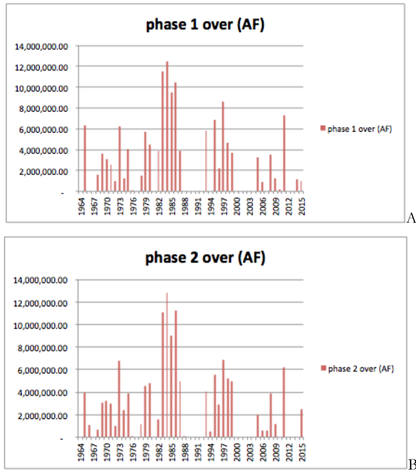
Figure 36. Graphs showing the volume of water in excess of 8.23 million af that would be transferred downstream under (A) Phase I and (B) Phase II of FMF, assuming that the inflow hydrology were the same as that which occurred between 1963 and 2016.
