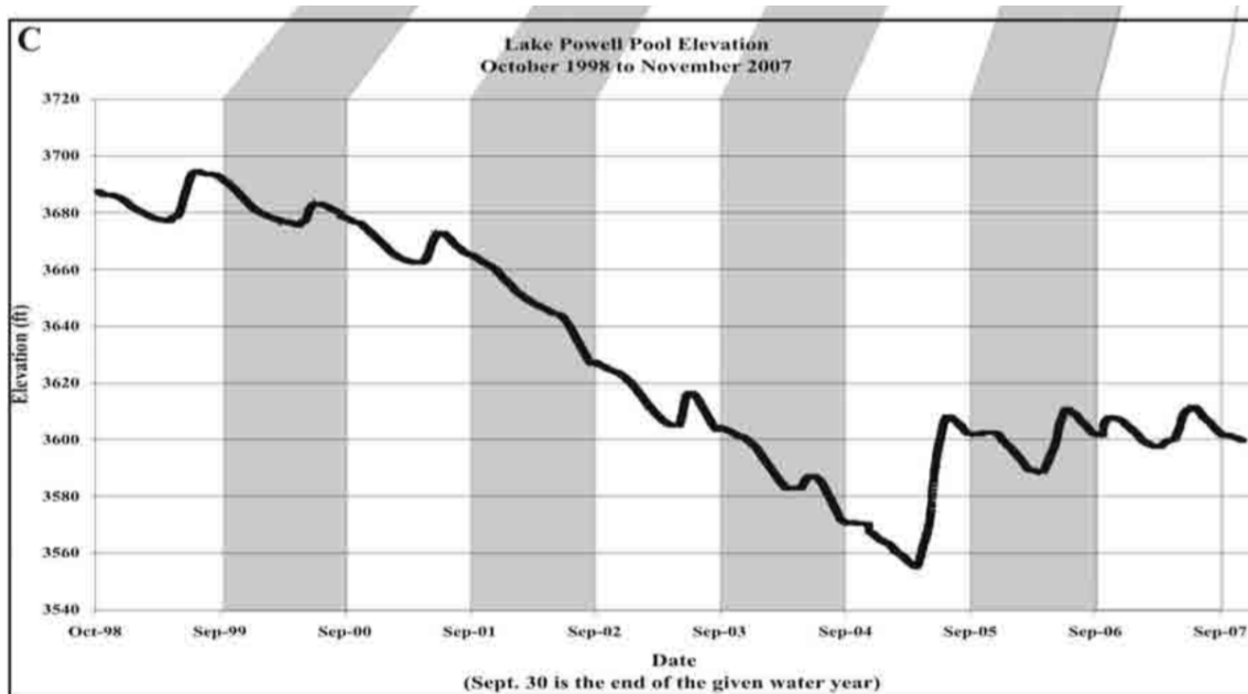
Figure 27. Graph showing elevation of Lake Powell during the period when bathymetric measurements described remobilization of fine sediment in the reservoir’s deltas (from Majeski, 2009, figure 1C).
