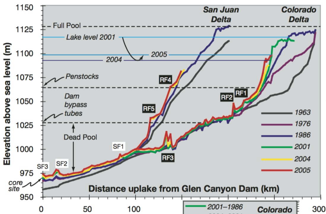
Figure 25. Graph showing the bathymetry along the centerline of the Colorado and San Juan arms of Lake Powell during successive surveys (Pratson et al., 2008, fig. 2A).
