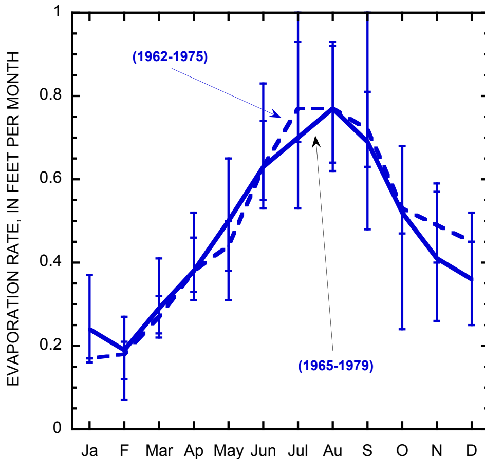
Figure 11. Graph showing monthly evaporation rates at Lake Powell as estimated by Jacoby et al (1977) for the period between 1962 and 1975 and by Reclamation (1986) between 1965 and 1979.
