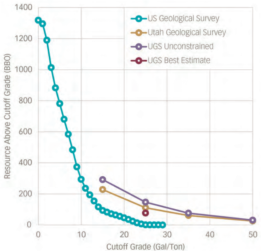
Figure 32: USGS and UGS Estimates of Oil Shale Resources in the Uinta Basin
