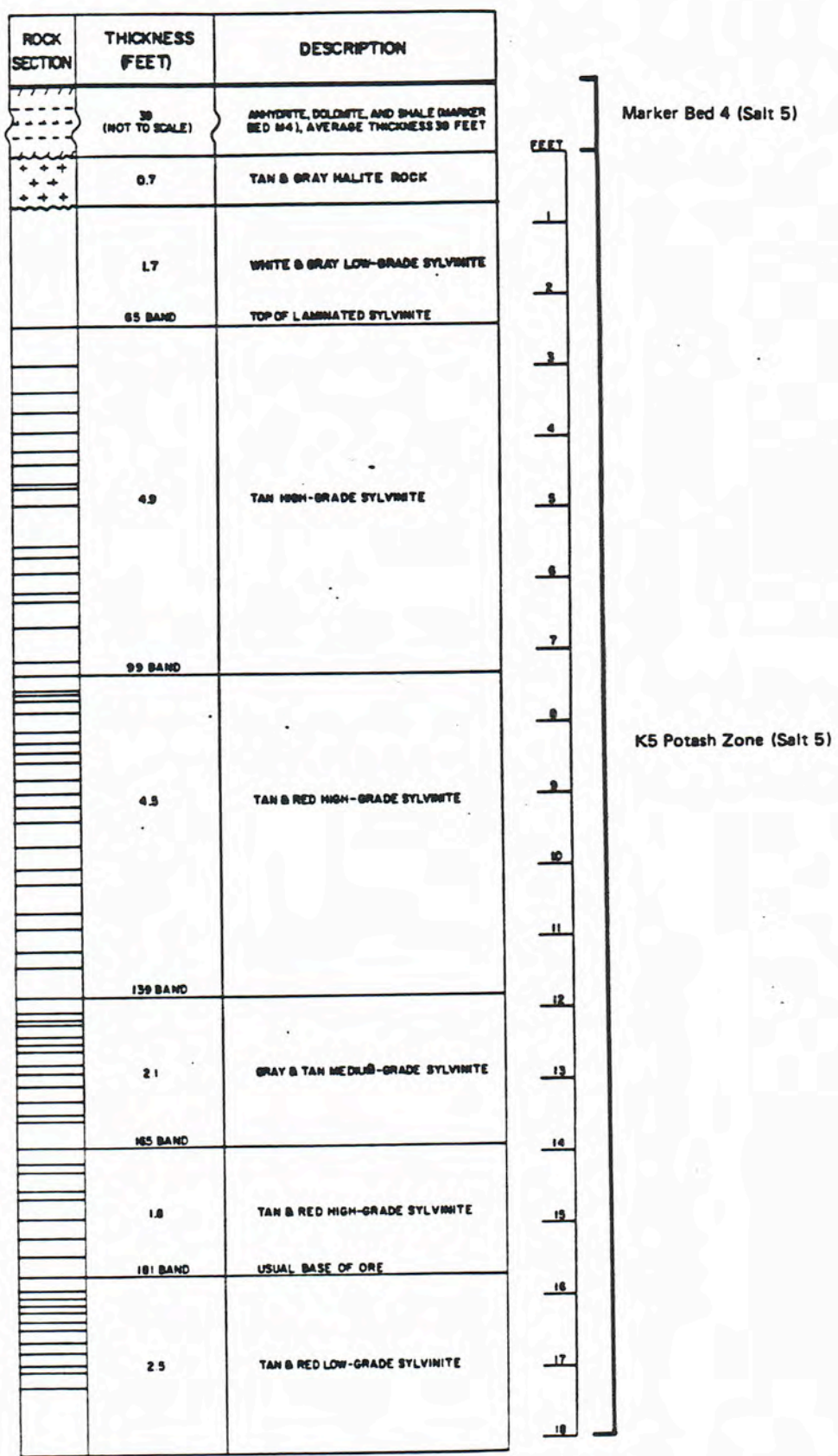
Figure 2. Stratigraphy of the K5 potash zone. Taken from Evans and Linn (1970, p. 289).
