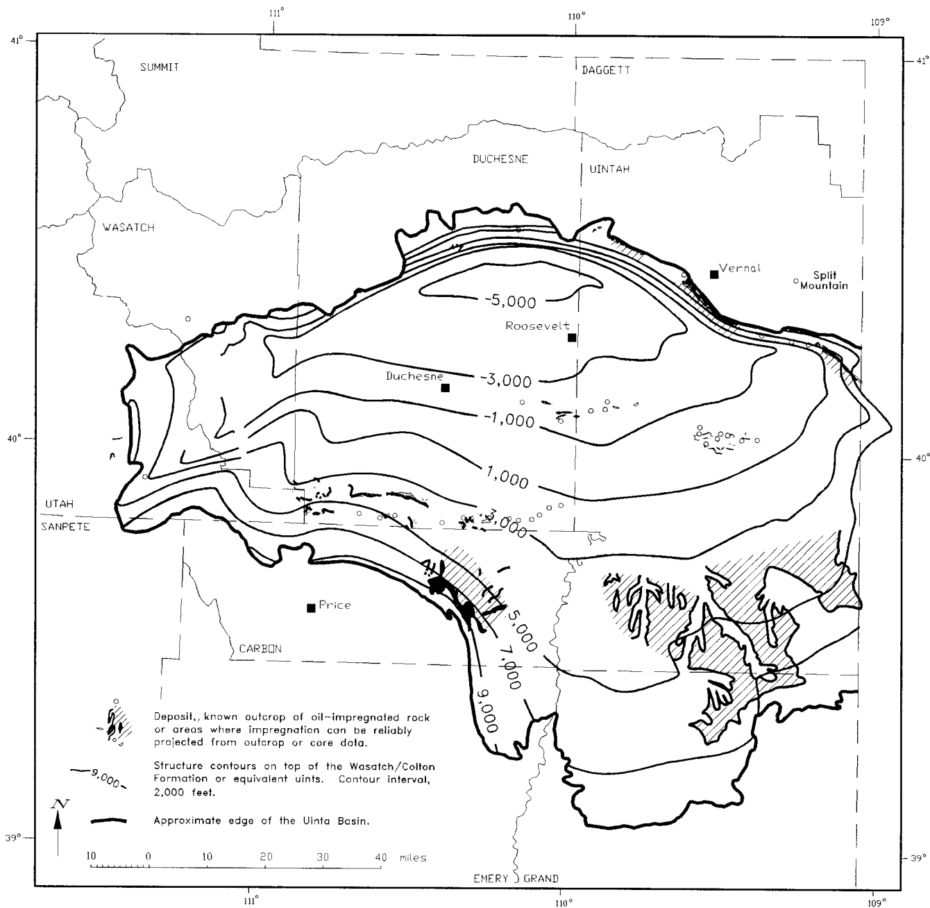
Figure 6. Structure contour map of the Uinta Basin. Contours are elevations, in feet above msl, of the top of the Wasatch/Colton Formation or equivalent units.
